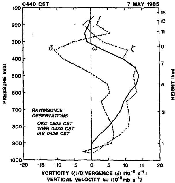
FIG.17. Kinematic analysis as in Fig. 12, except for mesovortex core at 0440 CST 7 May 1985.
