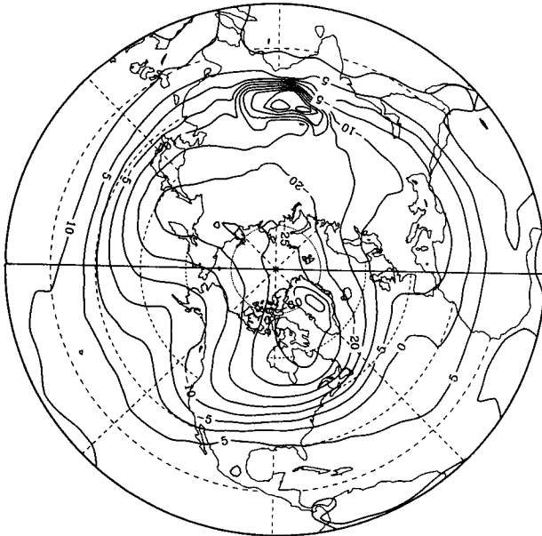
700 mb T Feb 1–15 1989
