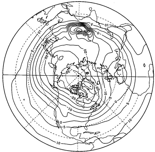
700 mb T Jan 16–31 1989
