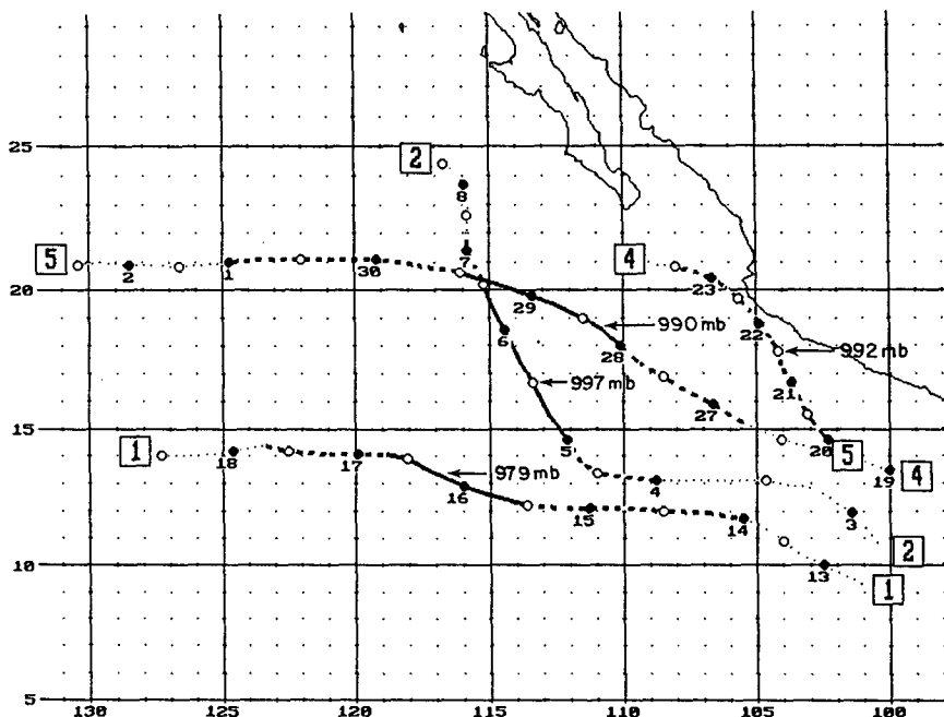
FIG. 1. (a), (b), (c), (d), (e), (f), and (g). Tropical storm and hurricane tracks of 1990.
