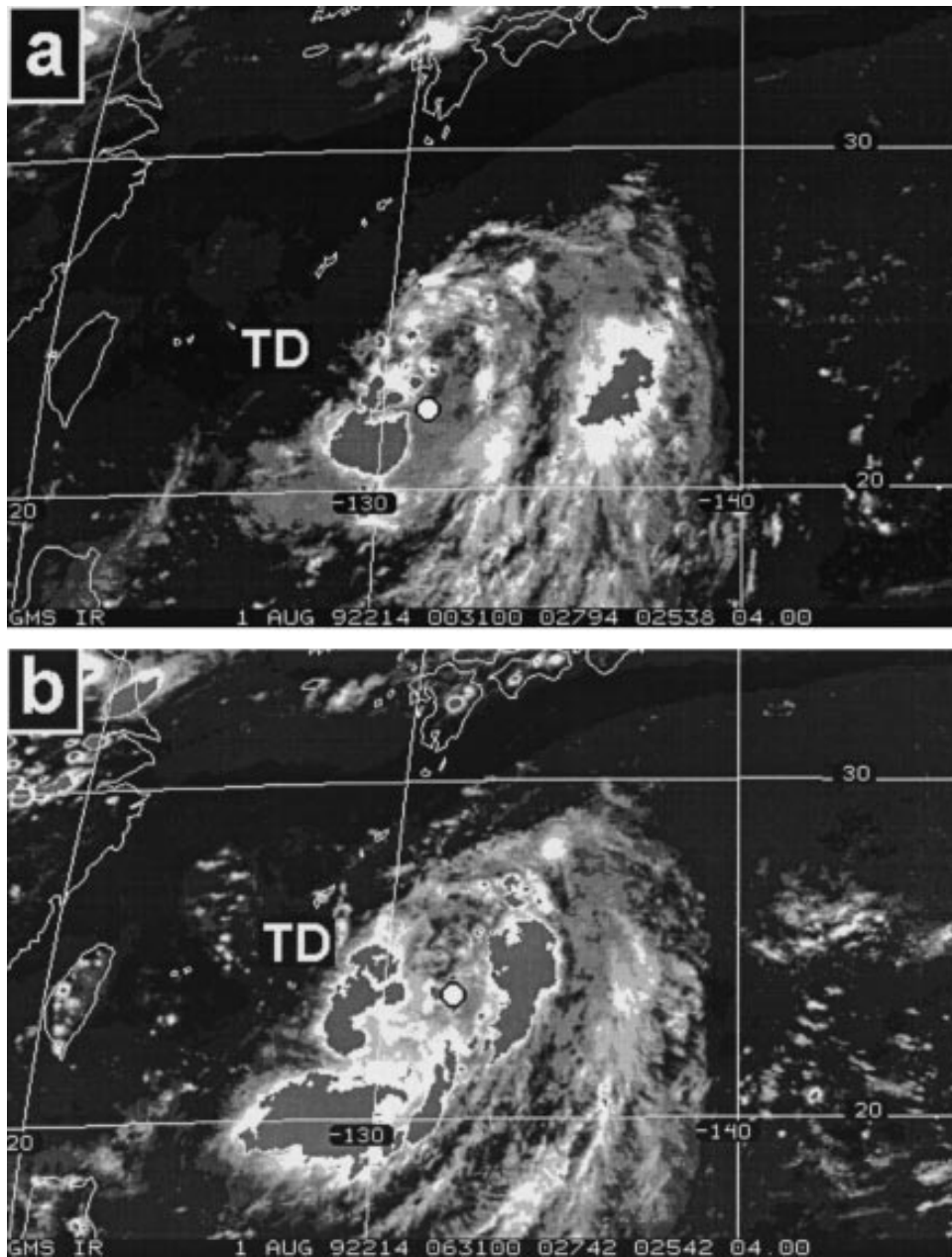
FIG. 8. Satellite imagery during the MCS–TD (tropical depression) interactions. JTWC positions are indicated by a circle: (a) 0000 UTC 1 August, (b) 0600 UTC 1 August, (c) 1200 UTC 1 August, (d) 1800 UTC 1 August, and (e) 0000 UTC 2 August.
