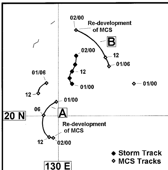
FIG. 9. Tracks of the storm and three MCSs during the interactions illustrated in the satellite imagery in Fig. 8. The A and B label corresponding vortices in Fig. 10. All times are UTC.
