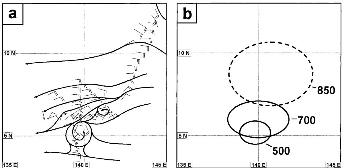
FIG. 5. (a) Streamline analysis of 500-hPa aircraft data for a 10-h period centered on 0000 UTC 24 July. (b) Relative sizes and positions of the 500-, 700-, and 850-hPa circulations as indicated in aircraft and surface data.
