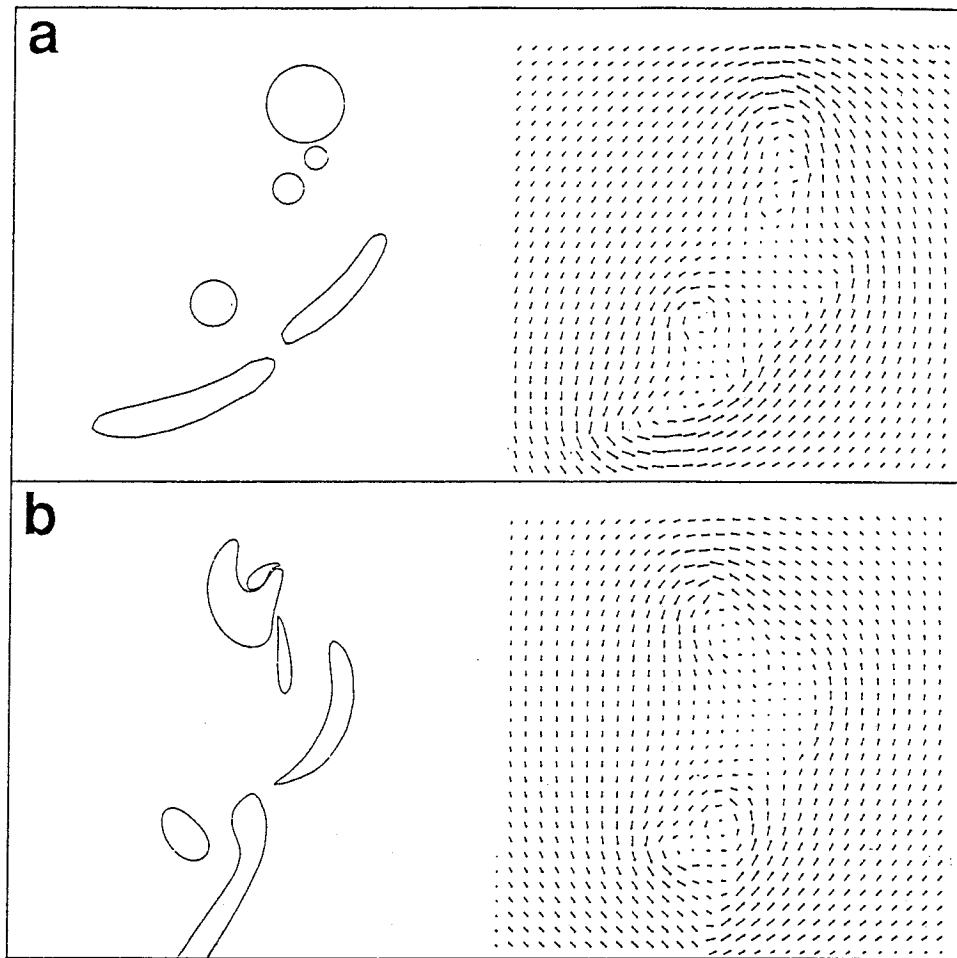
FIG. 11. Vortex patches and associated wind field for 2D simulation of MCS interactions in Typhoon Irving: (a) t = 0 and (b) t = 10 . All space and time variables are nondimensional.
