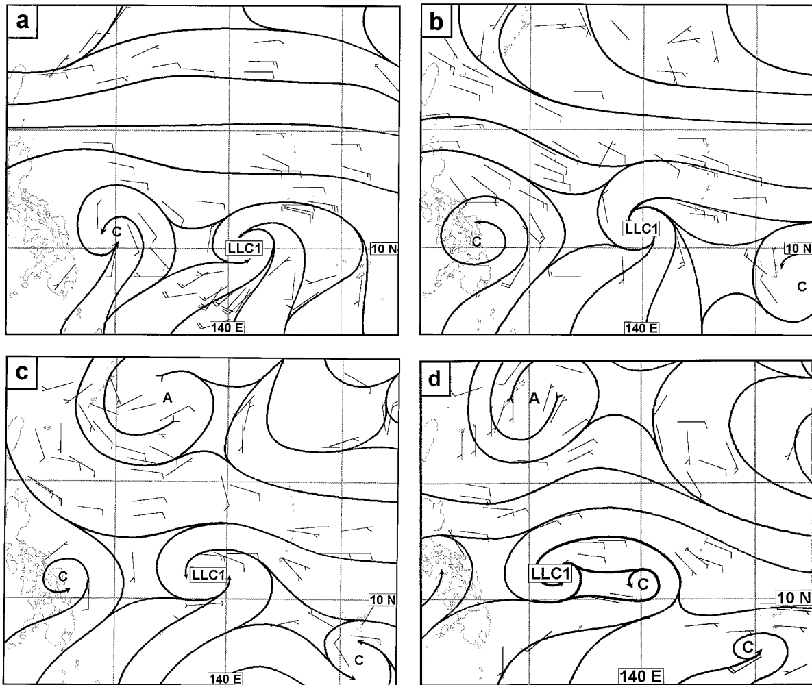
FIG. 2. Manual surface streamline analyses at 0000 UTC for the period 24–31 July 1992: (a) 24 July, (b) 25 July, (c) 26 July, (d) 27 July, (e) 28 July, (f) 29 July, (g) 30 July, and (h) 31 July. The low-level circulation initially located near 140°E is labeled LLC1. Latitude and longitude lines are plotted at 10° intervals. A full wind barb is 5 m s -1 .
