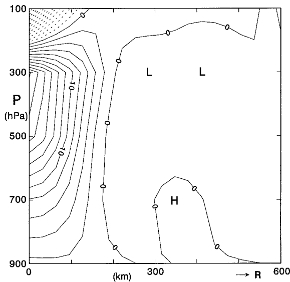
FIG. 13. Azimuthal average of relative vorticity at 120 h of integration for the interaction in Fig. 12, with an additional invariant background rotation similar to a monsoon trough structure. Contour intervals are 2.0 \times 10^{-5} \text{ s}^{-1} .
