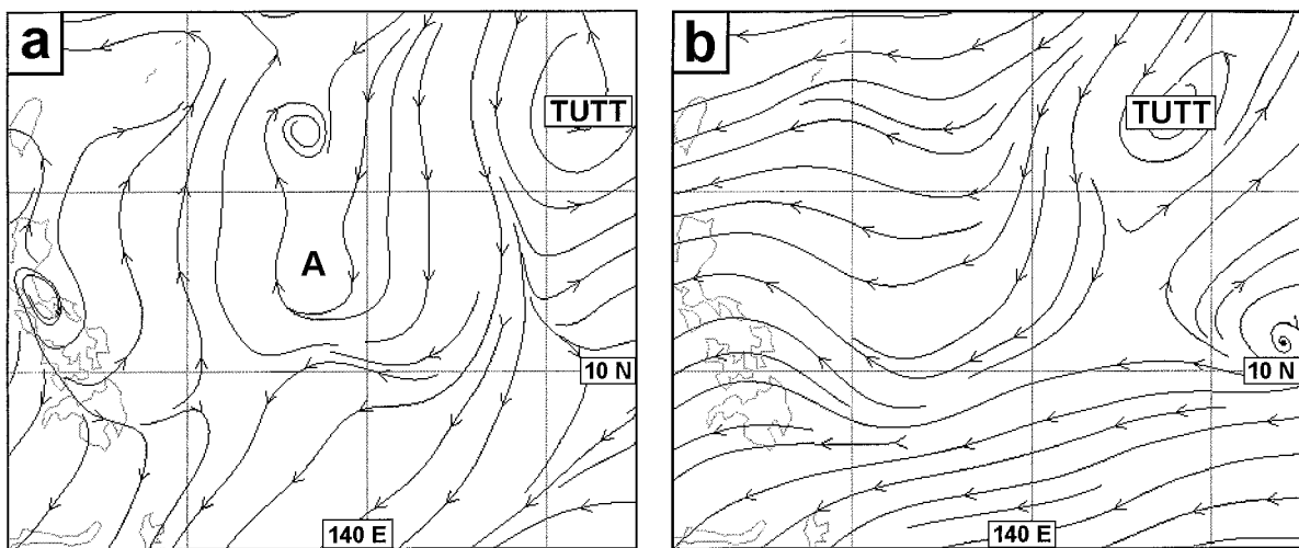
FIG. 3. Streamline analyses at 250 hPa for 0000 UTC from the Tropical Analysis System: (a) 25 July 1992 and (b) 27 July 1992.
