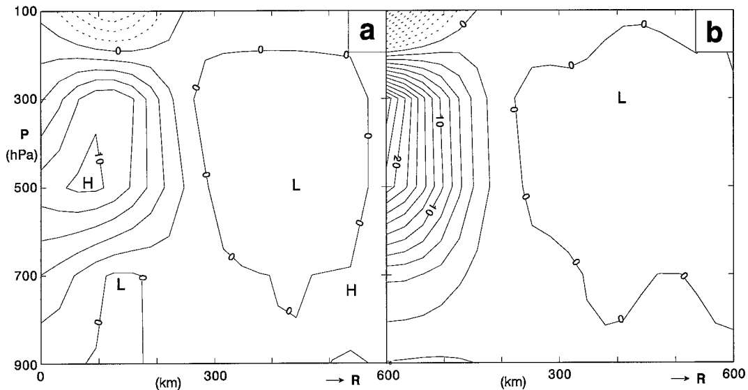
FIG. 12. Baroclinic model simulation of the interaction between two equal midlevel vortices: (a) Azimuthal average of relative vorticity at the initial time. (b) Azimuthal average of relative vorticity for the merged vortex at 72 h of integration. Contour intervals are 2.0 \times 10^{-5} \text{ s}^{-1} .
