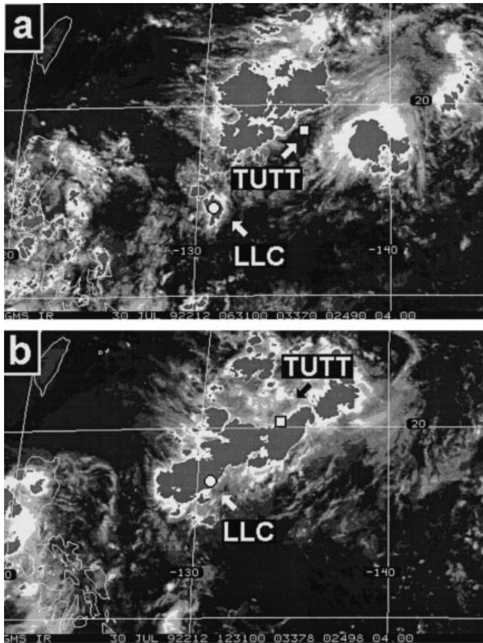
FIG. 7. Satellite imagery of the interaction between the low-level pre-Irving circulation ( \odot ) and the midlevel circulation associated with the TUTT ( \square ): (a) 0600 UTC 30 July, (b) 1200 UTC 30 July, (c) 2100 UTC 30 July, and (d) 0000 UTC 31 July.
