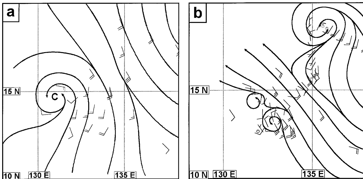
FIG. 6. Streamline analysis of aircraft data for a 10-h period centered near 0000 UTC 30 July: (a) 850 and (b) 500 hPa.
