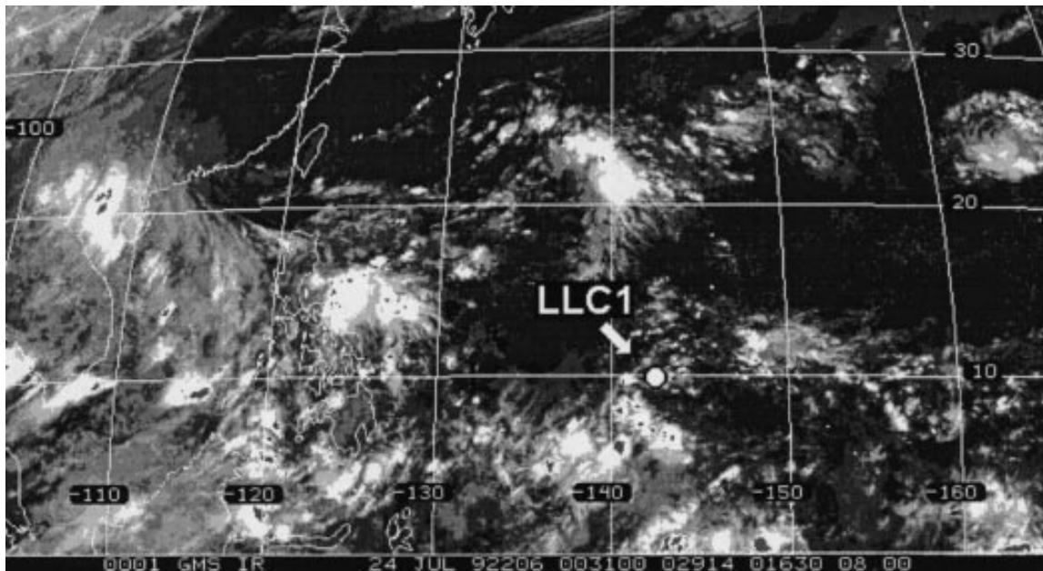
FIG. 4. Satellite imagery for 0000 UTC 24 July for the western North Pacific region. The circle indicates the position of LLC1.
