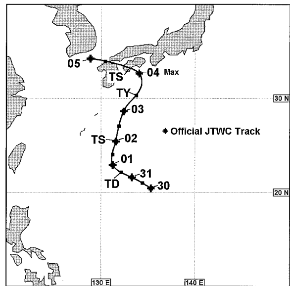
FIG. 1. The official JTWC track of Typhoon Irving. All times are UTC.
