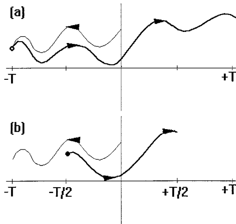
FIG. 1. Schematic illustration of original and modified filtering procedures. Thin lines indicate backward adiabatic integrations; thick lines indicate forward diabatic integrations. (a) Scheme of Huang and Lynch (1993): adiabatic step is not filtered. (b) Modified scheme: both steps are filtered.
