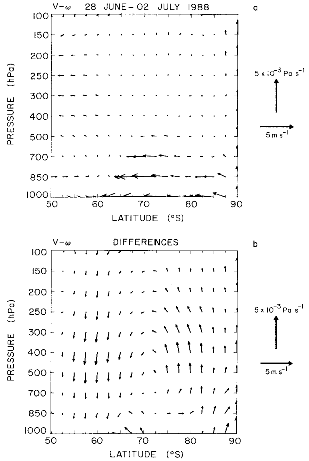
FIG. 7. (a) Mean meridional cross section of v components ( m s^{-1} ) and vertical velocities ( Pa s^{-1} \times -1000 ) in vector form, based on ECMWF 12-h analyses from 0000 UTC 28 June to 0000 UTC 2 July 1988. (b) Mean vector differences from the mean June–July 1988 representation in Fig. 5b.
