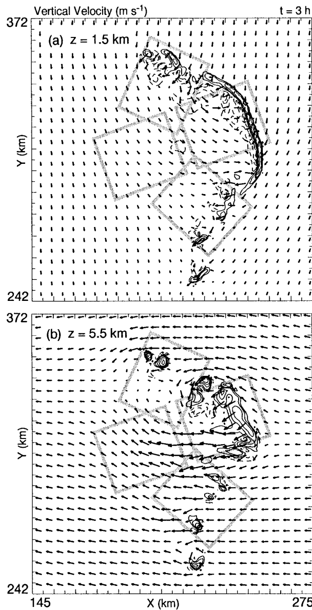
FIG. 8. Vertical velocity contoured at 1 and 2.5 m s^{-1} values, with additional positive values contoured in increments of 2.5 m s^{-1} (solid), and with negative values contoured at -0.5 , -1.0 , -1.5 , and -2.0 m s^{-1} (dashed) for 3 h at (a) 1.5 and (b) 5.5 km MSL. System-relative horizontal flow vectors are plotted with a vector the length of the space between tick marks having a magnitude of 10 m s^{-1} . The rectangles represent the location of the regional domains as in Fig. 3.
