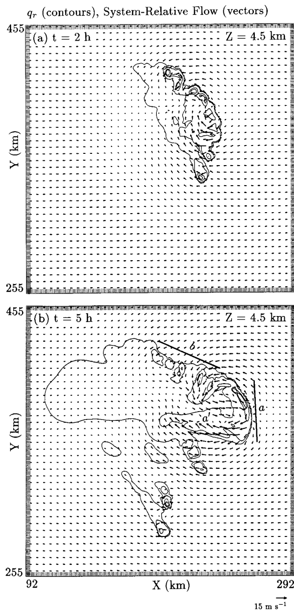
FIG. 2. The 4.5-km MSL rain field ( 0.01, 1, 2, 3, and 4 \text{ g kg}^{-1} contours) and system-relative wind vectors over the 200 \text{ km} \times 200 \text{ km} MCS-scale domain at (a) 2 h and (b) 5 h. In (b), the annotations indicate the precipitation features referred to in the text.
