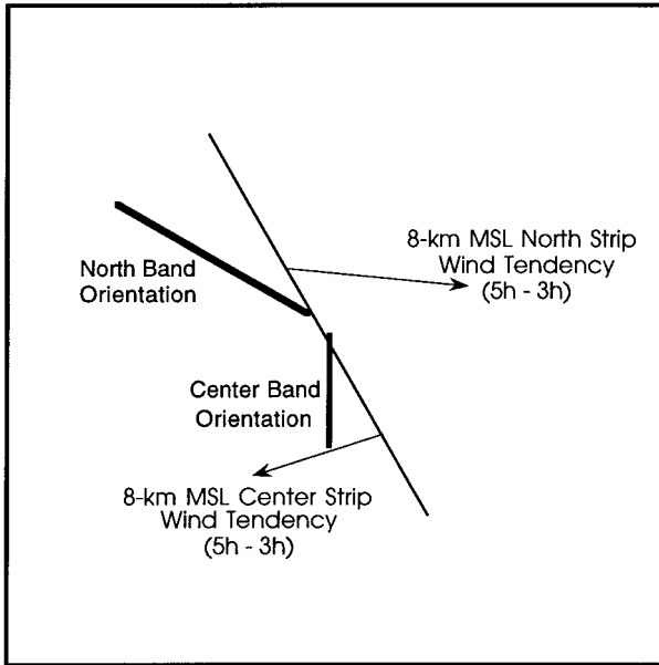
FIG. 14. Schematic diagram of the relationship between convective band orientation (bold solid lines) and the 8-km MSL regional accelerations from 3 to 5 h (thin arrows) in the 200 km × 40 km north and center strips displayed in Fig. 12.
