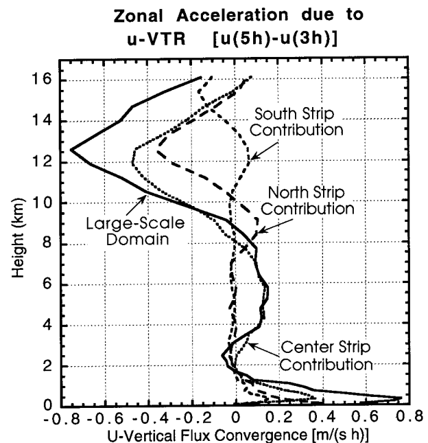
FIG. 18. Vertical profiles of the contribution of the horizontally averaged tendency of relative zonal momentum ( m s^{-1} h^{-1} ) from the vertical flux convergence term ( u -VTR) in Eq. (3) averaged from 3 to 5 h over the 200 km \times 200 km MCS-scale domain displayed in Figs. 2 and 12 (solid) and the contribution to this MCS-scale average from the north (large dash), south (medium dash), and center (small dash) 200 km \times 40 km subdomains displayed in Fig. 12.
