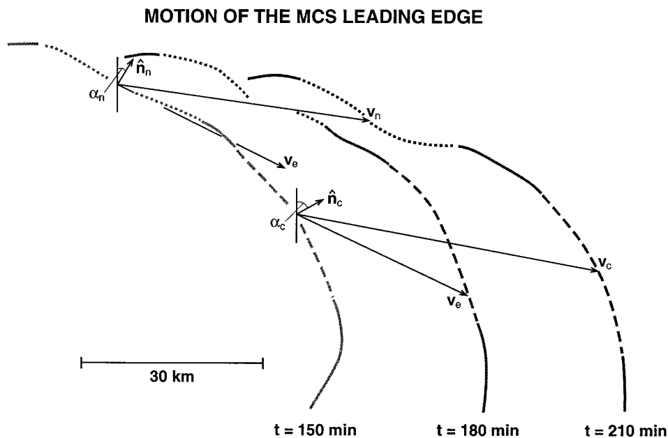
FIG. 5. Diagram indicating the respective earth-relative velocities \mathbf{V}_n and \mathbf{V}_c (long arrows) of the northern (dotted) and central (dashed) cold-pool edges from 150 to 210 min, and the relationship of these motions to both the respective local orientation vectors \hat{\mathbf{n}}_n and \hat{\mathbf{n}}_c (short arrows) of the northern and central cold-pool edges and the density-weighted mean environmental flow \mathbf{V}_e (long arrow) determined from the initial hodograph of Fig. 1b. The angle \alpha of the cold-pool orientation vector \hat{\mathbf{n}} is measured clockwise from the north. The velocity vectors \mathbf{V}_n , \mathbf{V}_c , and \mathbf{V}_e are scaled to represent distance traveled in the 1-h time increment at these constant velocities. The positions of the leading edge of the cold pool at 150, 180, and 210 min (indicated by the gray shading of variable intensity) are determined by the -0.01 \text{ m s}^{-2} buoyancy contour at 500 m MSL, with buoyancy defined as in Eq. (1) of Trier et al. (1997).
