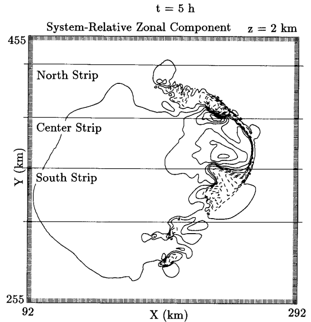
FIG. 12. The 2-km MSL relative zonal momentum at 5 h over the 200 km × 200 km large-scale domain of Fig. 2 contoured in intervals of 2 m s -1 . The 200 km × 40 km strips signify the north, center, and southern subdomains over which separate contributions to the averages presented in Fig. 13 are computed. Positive values are solid; negative values are dashed.
