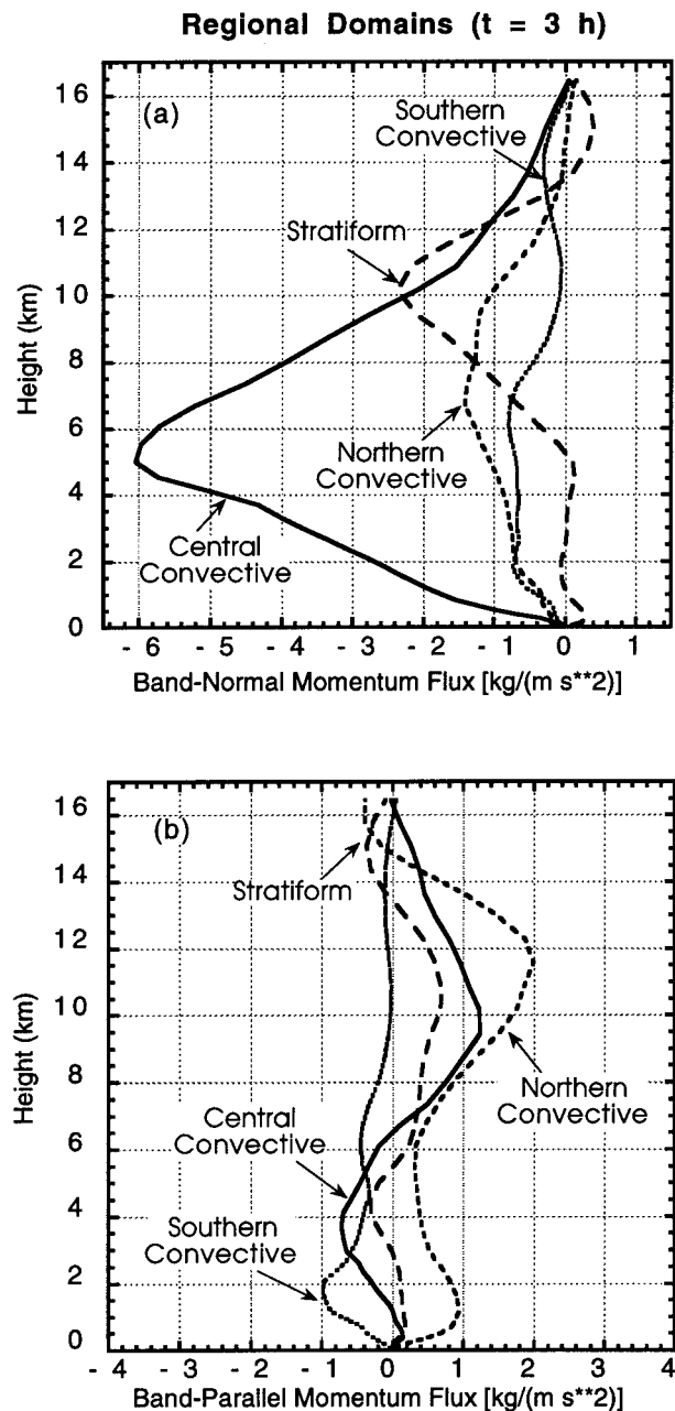
FIG. 9. Vertical profiles of the vertical flux of the relative horizontal momentum ( kg m^{-1} s^{-2} ) oriented (a) normal and (b) parallel to the leading-edge convective band at 3 h for the regional domains displayed in Fig. 3.
