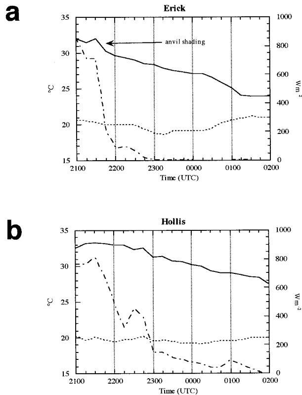
FIG. 9. Time series of temperature (solid) and dewpoint (dashed), both in °C, and incoming solar shortwave radiation (dash-dot trace), in W m -2 , from 2100 to 0200 UTC 22–23 May 1995 for (a) Erick and (b) Hollis, OK. See Fig. 3f for the locations of these sites.
