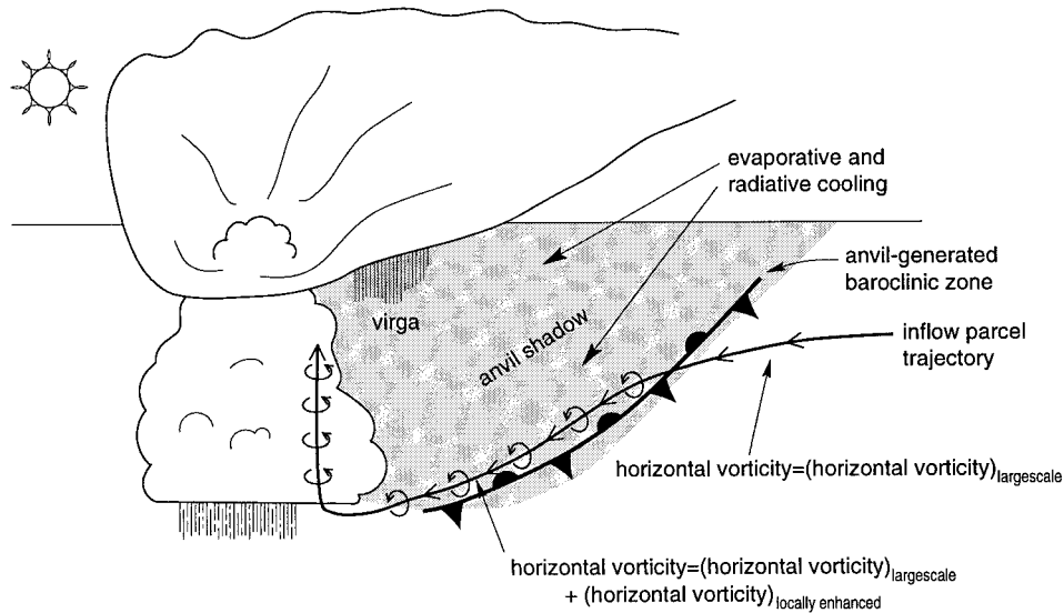
FIG. 1. A conceptual model for the enhancement of low-level horizontal vorticity by an anvil-generated baroclinic zone. The amount of horizontal vorticity generated is a function of baroclinity and parcel residence time in the baroclinic zone. Residence time is a function of both storm-relative inflow speed and crossing angle with respect to the baroclinity.
