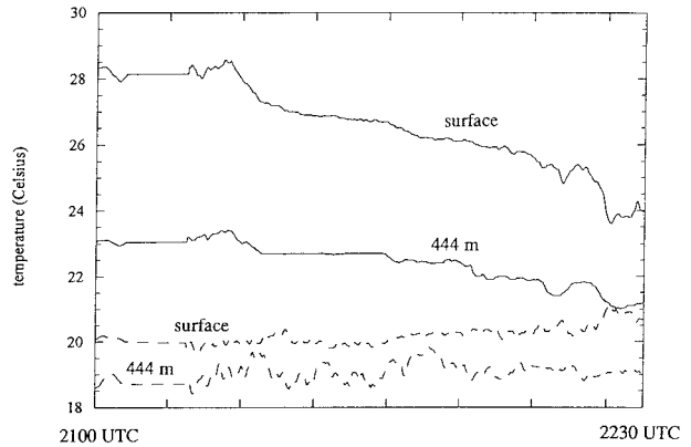
FIG. 14. Time series of temperature (solid, ^{\circ}\text{C} ) and dewpoint (dashed, ^{\circ}\text{C} ) measured by the instrumented tower between 2100 and 2230 UTC on 17 May 1981. The heights of the measurements are indicated.
