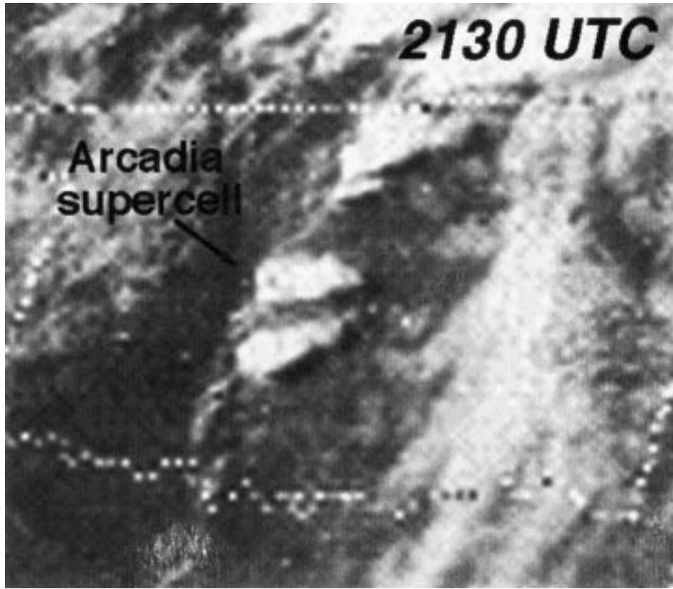
FIG. 12. Visible satellite image at 2130 UTC 17 May 1981.
