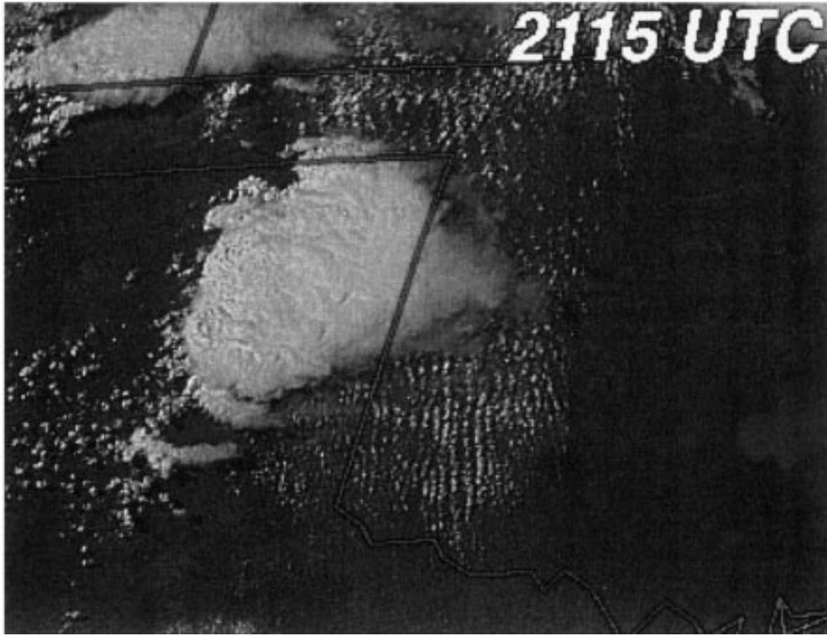
FIG. 7. High-resolution GOES-8 visible satellite imagery for (a) 2115 and (b) 2315 UTC 22 May 1995. The relatively isolated storm in (b), whose updraft and overshooting top lies in the eastern Texas panhandle, was a nontornadic supercell.
