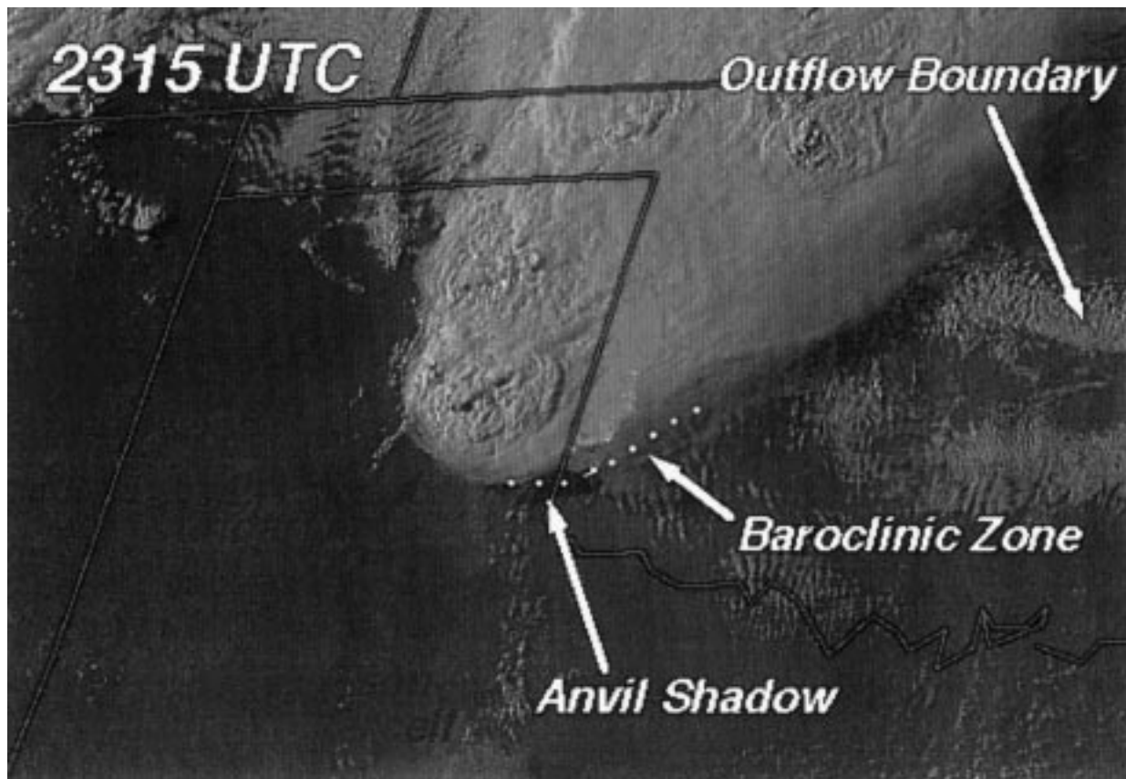
FIG. 2. High-resolution GOES-8 visible satellite imagery for 2315 UTC 8 June 1995. Strong insolation is reaching the surface south of the anvil edges of the supercell that spawned violent tornadoes near Kellerville and Allison, TX.
