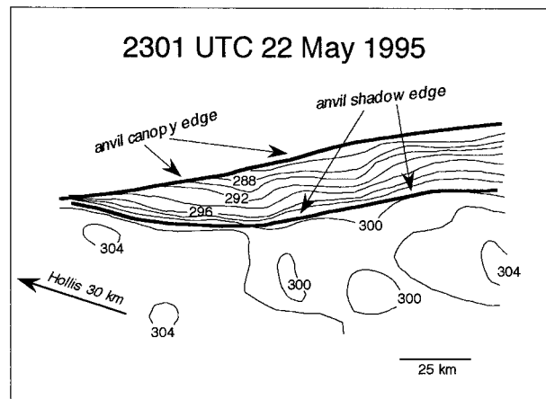
FIG. 10. Skin temperatures at 2301 UTC 22 May 1995 in southwestern Oklahoma near the anvil shadow edge, as determined from GOES-8. Isotherms are contoured at 2-K intervals.
