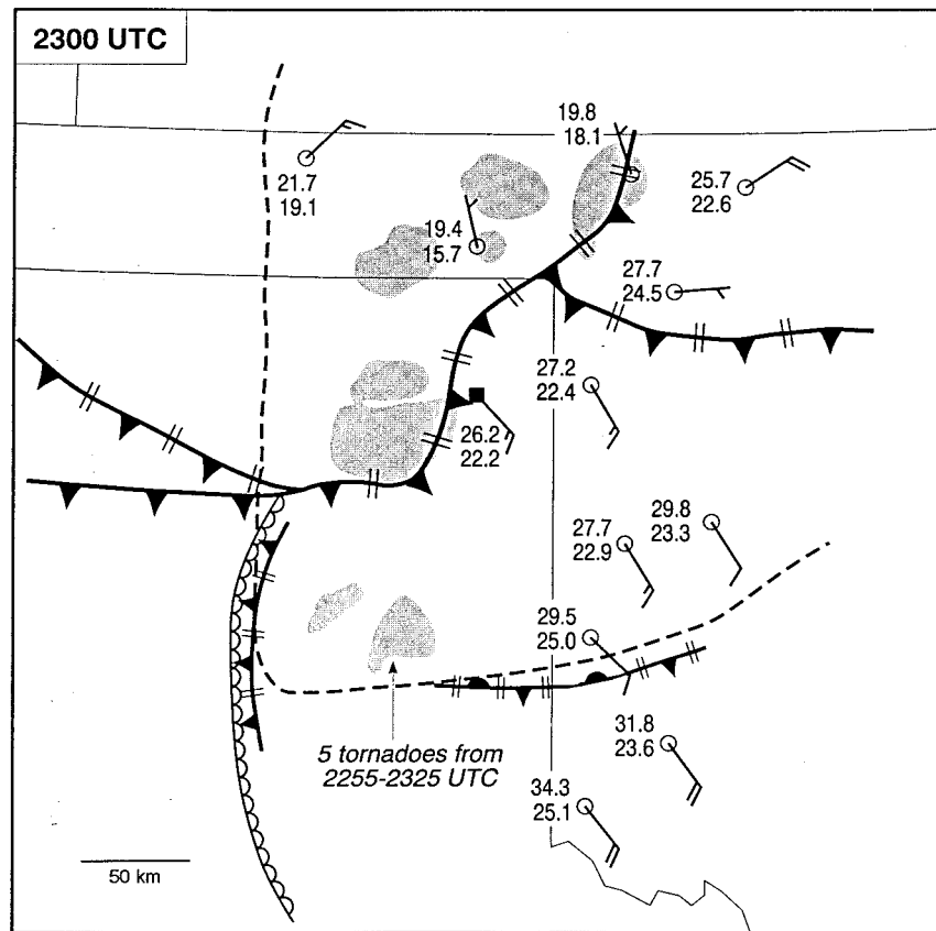
FIG. 5. Mesoscale analysis for 2300 UTC 8 June 1995. Each full wind barb represents 5 \text{ m s}^{-1} . Temperatures and dewpoints are shown in ^{\circ}\text{C} . The open-circled surface observations are from the Oklahoma Mesonet, and the filled square observation is a VORTEX mobile mesonet observation. Radar echoes >35 \text{ dBZ} are shaded. Fronts are denoted by conventional symbols; however, mesoscale fronts, e.g., outflow boundaries and the anvil-generated baroclinic zone, are depicted using the symbology of Young and Fritsch (1989). The dryline is depicted by the unfilled scalloped line. The anvil canopy edge is depicted by the dashed line.
