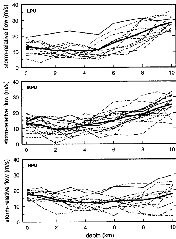
FIG. 9. Storm-relative (SR) wind speed ( \text{m s}^{-1} ) for all cases. The top graph is for LP storms, the middle for CL storms, and the bottom for HP storms. Heavy curves represent the mean for each storm type.
