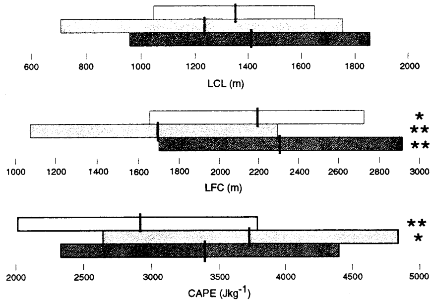
FIG. 4. Bar graphs of the distributions of LCL height (m AGL), LFC height (m AGL), and CAPE ( J kg^{-1} ). The black vertical ticks at the center of each bar are at the mean value, and the bar extends \pm 1 standard deviation from the mean. A single asterisk beside the bar indicates that the mean is significantly different than all supercells at the 95% confidence level, and a double-asterisk indicates significance at the 98% confidence level. The white bar is for LP storms, gray for CL, and dark gray for HP.
