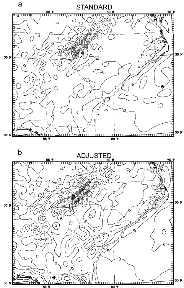
FIG. 8. Moisture divergence at 1600 EST at \sigma = 0.985 (about 150 m above ground) from the (a) standard and (b) adjusted model forecasts. Contours are at intervals of 6 \times 10^{-7} \text{ s}^{-1} .
