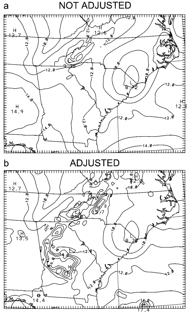
FIG. 2. Water vapor mixing ratios ( \text{g kg}^{-1} ) from the model (a) before (1000 EST) and (b) after (1005 EST) the humidity adjustment. The area shown is the fine-grid model domain, but having excluded the outer four rows and columns.
