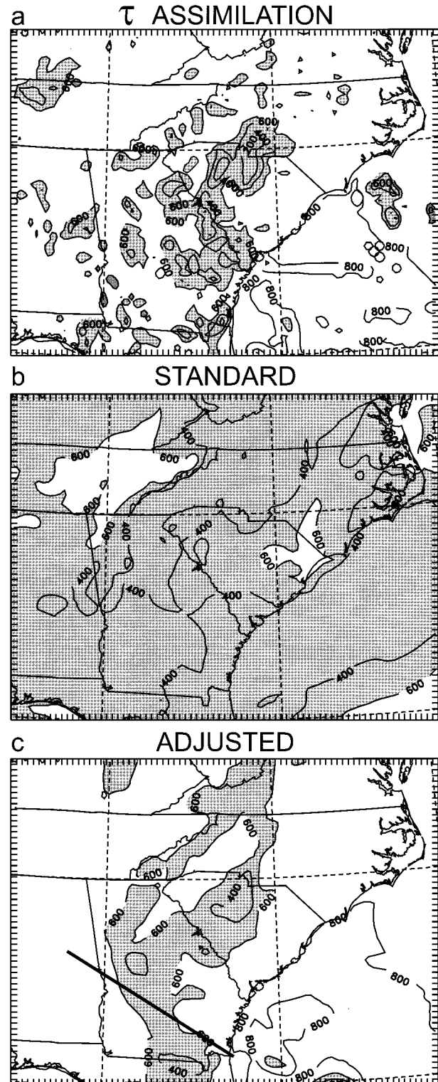
FIG. 6. Surface insolation ( \text{W m}^{-2} ) at 1300 EST from (a) the reference field, as defined in the text; (b) the forecast with the standard model; and (c) the adjusted forecast. Areas with values < 600 \text{ W m}^{-2} are shaded gray. The thick solid line in (c) indicates the location of the cross section in Fig. 7.
