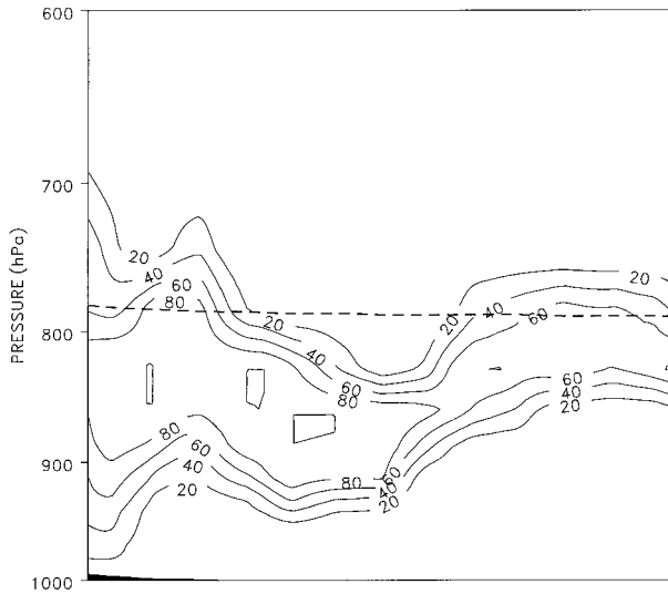
FIG. 4. A cross section of the cloud fraction (%), as retrieved from 1000 EST satellite data. The dashed line is the border ( \sigma surface) between zones identified with low and middle clouds in the model. The cross section goes from northwest (left) to southeast (right) along the line marked in Fig. 3b.
