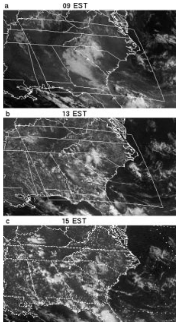
FIG. 1. GOES visible satellite images at (a) 0900, (b) 1300, and (c) 1500 EST 23 Aug 1993. The analysis domain is outlined in (a) and (b). Panel (c) was generated from a different data archive than (a) and (b), with a coarser image resolution.
