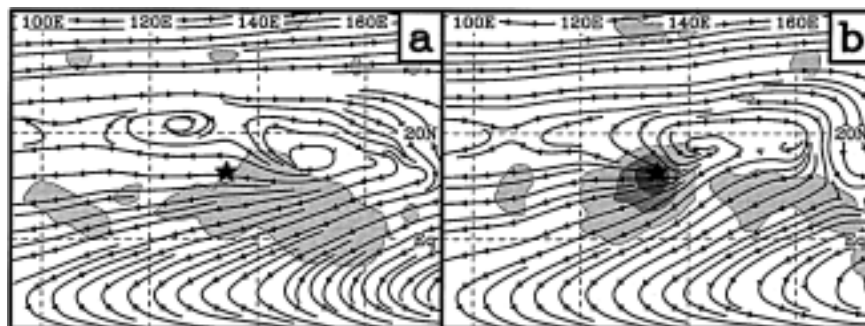
FIG. 6. Composite streamline and divergence fields at 250 hPa for the monsoon shear line pattern for (a) -72 and (b) 0 \text{ h} . The contour interval is 2.5 \times 10^{-6} \text{ s}^{-1} with shading indicating regions greater than 2.5 \times 10^{-6} \text{ s}^{-1} . The mean genesis location ( \star ) and lat-long lines are marked for reference.
