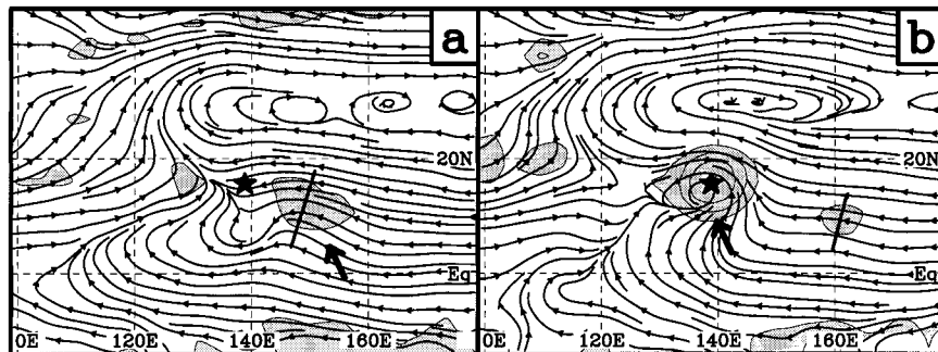
FIG. 3. Composite streamline and cyclonic relative vorticity fields at 700 hPa for all Jul genesis events over the 8-yr study period at (a) –72 and (b) 0 h. Contours and shading indicate values of relative vorticity greater than 4 \times 10^{-6} \text{ s}^{-1} . The mean genesis location (*) and lat–long lines are marked for reference.
