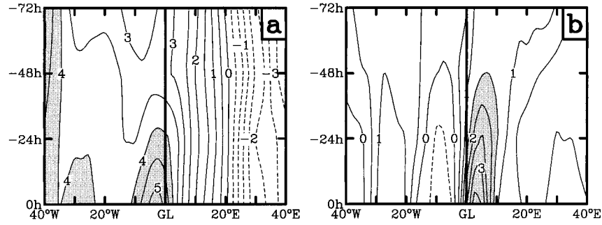
FIG. 7. Time-longitude diagram at 850 hPa for the monsoon shear line composite for (a) zonal wind component with shading indicating values greater than 4.0 \text{ m s}^{-1} and (b) meridional wind component with shading indicating values greater than 1.5 \text{ m s}^{-1} . The components are averaged over a 7.5^\circ lat strip equatorward of the genesis location (GL).
