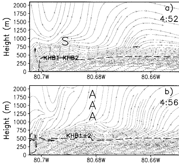
FIG. 20. (a) Trajectory source region at 4:52 and (b) arrival locations at 4:56. Point S denotes source region in (a), while A denotes arrival locations in (b). The u-w streamlines also are shown.
