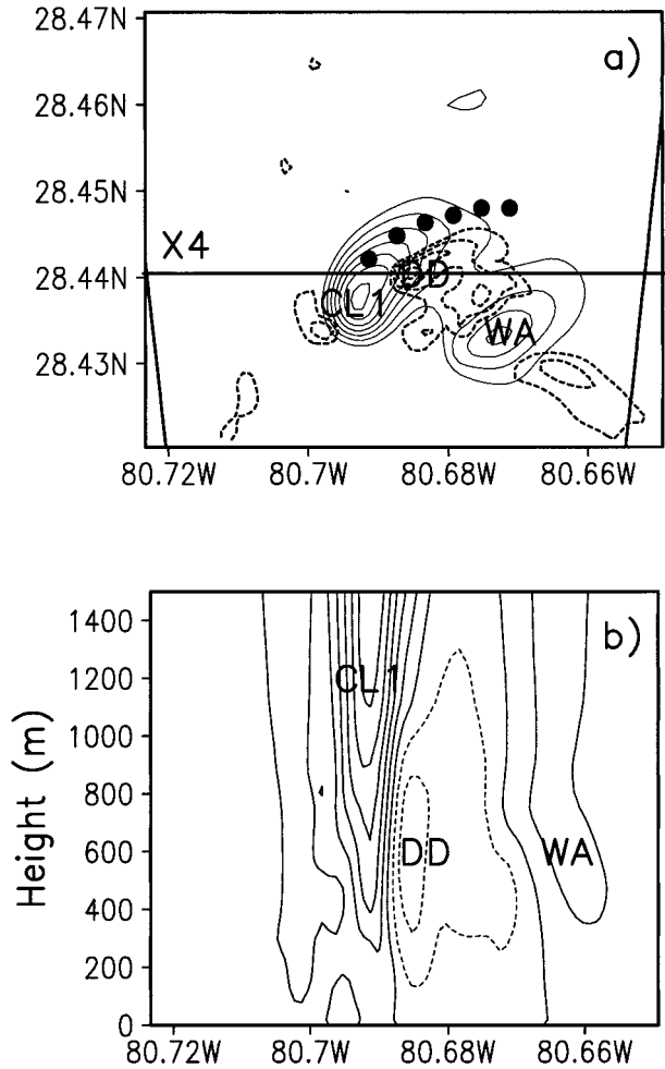
FIG. 10. (a) Upward vertical motion (solid) at 2.1 km above the surface at 4:56. Also shown is the downward vertical motion (dashed) at 500 m above the surface. Contours range from -8 to 14 \text{ m s}^{-1} , with an interval of 2 \text{ m s}^{-1} . CL1 indicates updraft of cell 1, while DD indicates the downdraft produced by CL1. Here, WA indicates position of weak ascent discussed in text. The thick dotted line indicates the surface position of OF1 at 4:56. (b) Cross section of vertical motion ( \text{m s}^{-1} ) denoted X4 in top panel. Values range from -6 to 15 \text{ m s}^{-1} , with an interval of 3 \text{ m s}^{-1} . CL1, DD, and WA indicate the same features as in the top panel.
