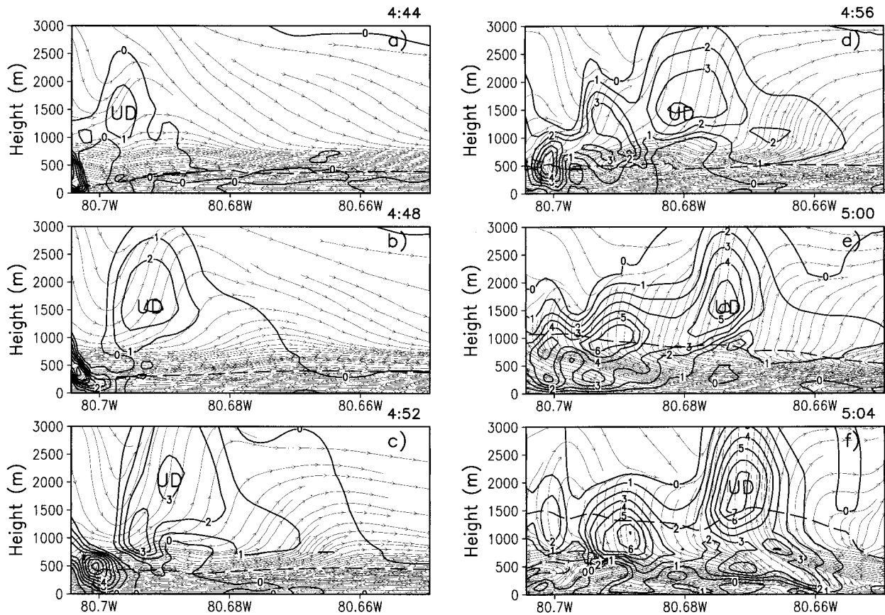
FIG. 15. As in Fig. 13 but including upward vertical motion (solid lines, \text{m s}^{-1} ). Also note the different vertical scale. Here UD indicates position of updraft discussed in text.
