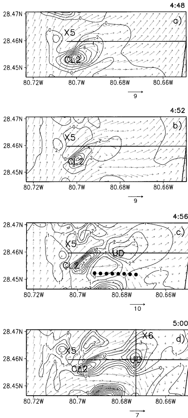
FIG. 16. Upward vertical motion ( m s^{-1} ) and winds at 1.5 km above the surface at (a) 4:48, (b) 4:52, (c) 4:56, and (d) 5:00. Contour interval in (a) and (b) is 2 m s^{-1} , while interval in (c) and (d) is 1 m s^{-1} . X5 indicates cross section discussed previously. CL2 denotes location of cell 2. Here UD corresponds to the updraft discussed in Fig. 15. X6 denotes cross section discussed in Fig. 21. Thick dotted line in (c) indicates surface position of OF3.
