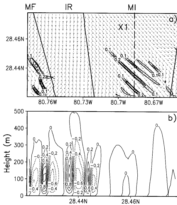
FIG. 5. (a) Upward vertical motion ( \text{m s}^{-1} ) and winds at 18 m above the surface within D3 at 2:36. (b) Cross section (denoted X1 in Fig. 5a) of vertical motion ( \text{m s}^{-1} ). MF denotes mainland Florida, while IR and MI denote locations of the Indian River and Merritt Island, respectively (see Fig. 1).
