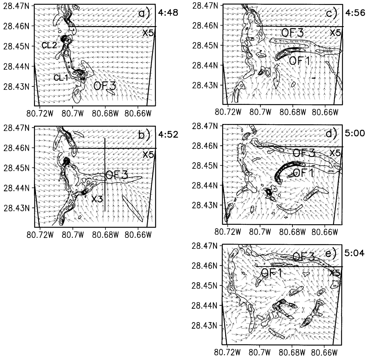
FIG. 8. Upward vertical motion ( \text{m s}^{-1} ) and winds at (a) 4:48, (b) 4:52, (c) 4:56, (d) 5:00, and (e) 5:04 at 88 m above the surface. Minimum contour is 1 \text{ m s}^{-1} . Contour interval is 1 \text{ m s}^{-1} . OF1 and OF3 indicate positions of outflow boundaries discussed in text. X5 denotes cross section discussed in Figs. 13 and 15. X3 denotes cross section discussed in Fig. 9.
