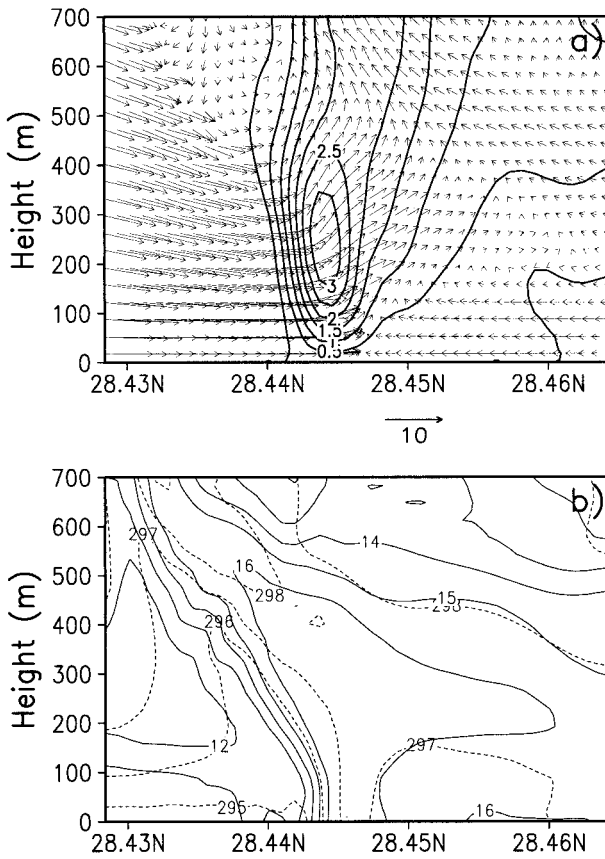
FIG. 9. (a) Upward vertical motion ( \text{m s}^{-1} ) and v-w windflow, and (b) potential temperature (K, dotted lines) and mixing ratio ( \text{g kg}^{-1} , solid lines) along X3 at 4:52. Axis of X3 is shown in Fig. 8b.
