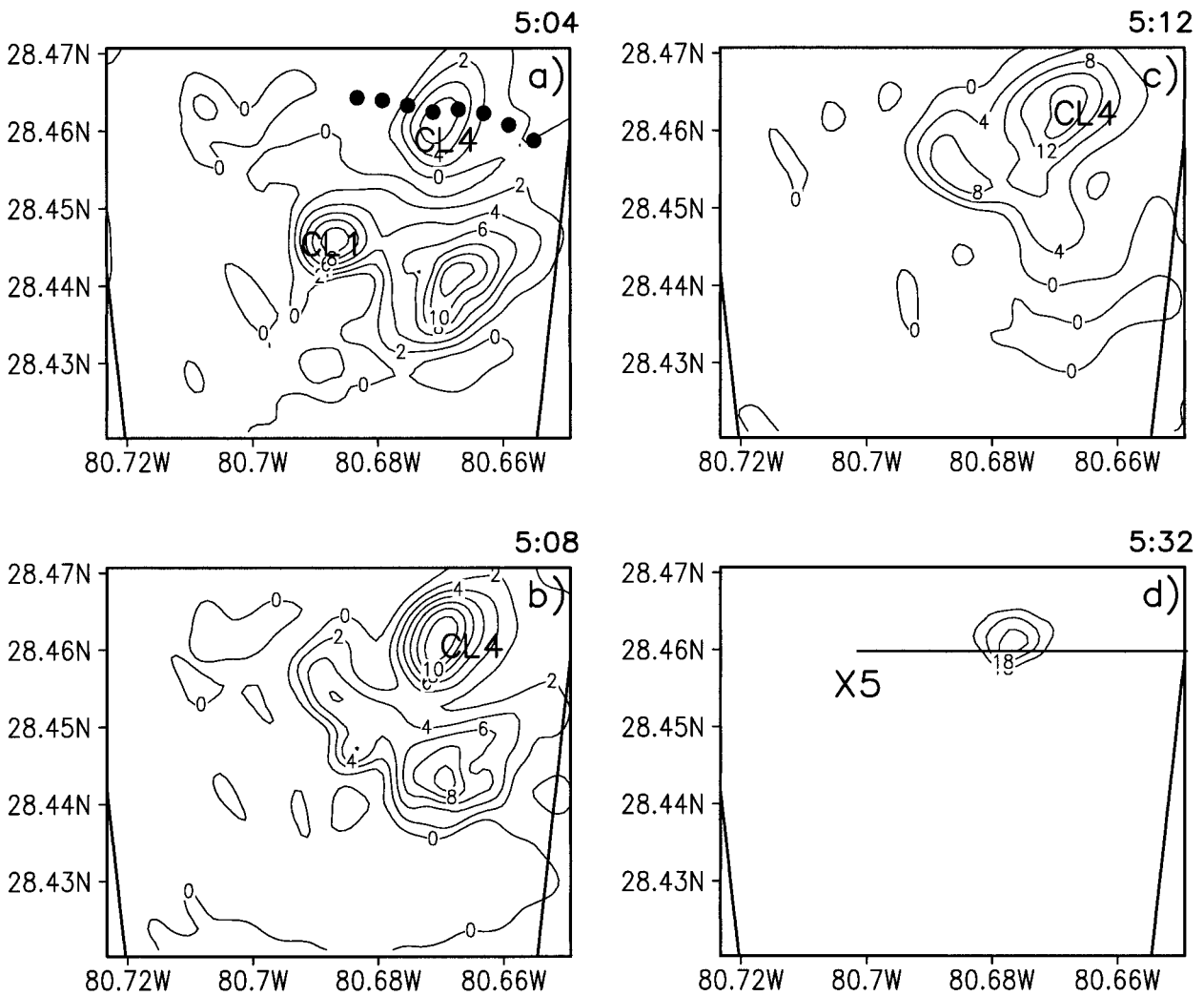
FIG. 12. Upward vertical motion ( \text{m s}^{-1} ) 2.1 km above the surface at (a) 5:04, (b) 5:08, and (c) 5:12. (d) Accumulated rainfall (mm) greater than 15 mm at 5:32. CL1 and CL4 indicate the positions of cell 1 and cell 4, respectively. The thick dotted line in (a) denotes the surface position of OF3 at 5:04. X5 in (d) indicates the location of the cross section discussed in Figs. 13 and 15.
