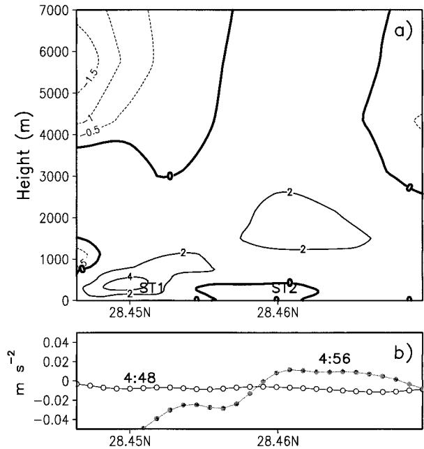
FIG. 21. (a) Cross section of the difference in vertical motion between 4:56 and 4:48 along X6 in Fig. 16d. Solid (dashed) lines indicate positive (negative) differences. Thick solid line denotes zero contour. Contour interval is 2 \text{ m s}^{-1} ( 0.5 \text{ m s}^{-1} ) for positive (negative) values. ST1 and ST2 correspond to skew T locations in Fig. 22. (b) Total buoyancy force ( \text{m s}^{-2} ) along X6 at 4.3 km above the surface at 4:48 (open dots) and 4:56 (filled dots).
