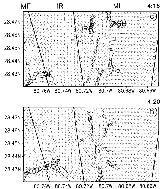
FIG. 6. Upward vertical motion ( \text{m s}^{-1} ) and winds at 18 m above the surface at (a) 4:16 and (b) 4:20. IRB, SB, and OF indicate positions of the Indian River breeze, sea breeze, and outflow boundary, respectively.
