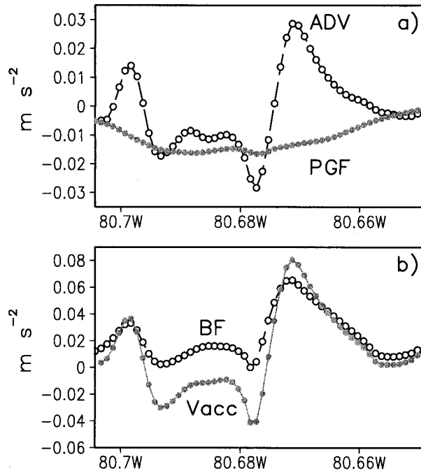
FIG. 17. (a) Three-dimensional ADV, PGF, and (b) BF and net vertical acceleration (Vacc) along X5 at 2.5 km above the surface at 5:00. All values are in m s^{-2} .
