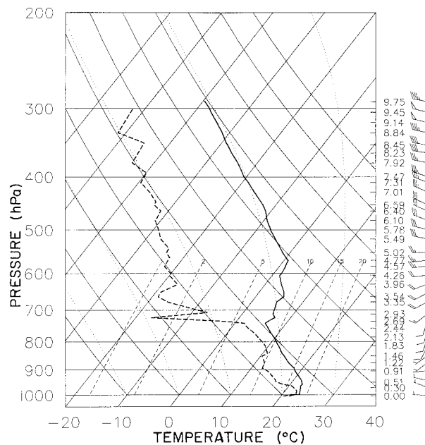
FIG. 3. Cape Canaveral sounding at 1000 UTC 4 Jun 1997 used in conjunction with the Meso-Eta analysis for model initialization. Wind barbs in m s -1 (half barb = 5 m s -1 ).
