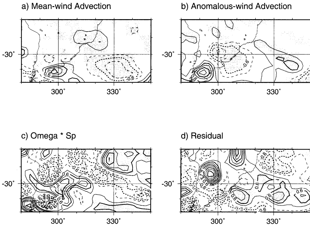
FIG. 5. Terms in the linearized quasigeostrophic thermodynamic equation at 850 hPa for the anomalously intense SACZ composite (see text): (a) -\bar{\mathbf{v}} \cdot \nabla \mathbf{T}' , (b) -\mathbf{v}' \cdot \nabla \bar{\mathbf{T}} , (c) S_p \omega' , and (d) R_T . The contour interval is 0.3 \times 10^{-5} \text{ K s}^{-1} ; zero contour omitted and negative dashed. Shaded areas are significant at the 95% confidence level, from a two-tailed Student's t -test with nine degrees of freedom.
