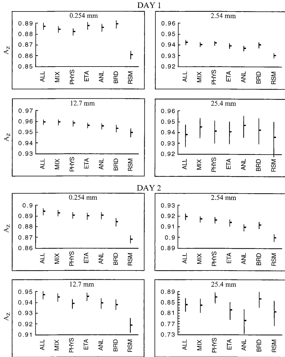
FIG. 14. Areas ( A_z ) under fitted ROC curves for all of the ensemble groups for the four precipitation thresholds: 0.254, 2.54, 12.7, and 25.4 mm, for day 1 and day 2 forecasts. Error bars are computed such that ensemble groups with nonoverlapping bars are significantly different with 95% confidence.
