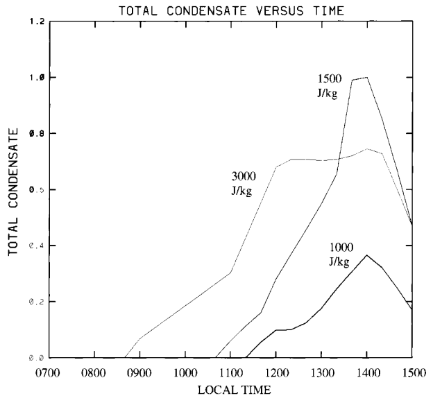
FIG. 15. Total condensate against time for simulations with upstream CAPEs of 1000, 1500, and 3000 J \text{kg}^{-1} . All measures are normalized by the maximum value from the control experiment.
