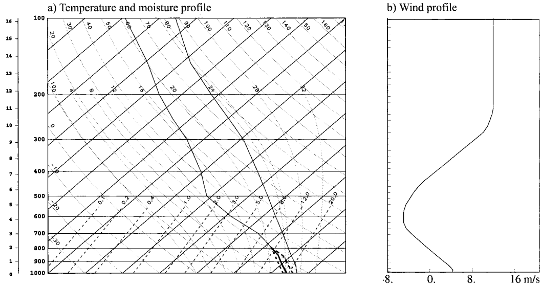
FIG. 3. (a) Temperature and moisture sounding used in the control experiment with the nonlinear model. Moisture profiles with CAPEs of 1000 J kg -1 (dotted) and 3000 J kg -1 (dashed) are also shown. (b) Wind profile.
