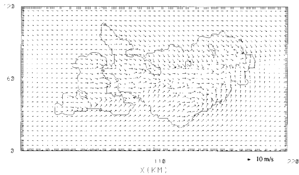
FIG. 4. Surface vectors at t = 1100 LT for a simulation without moisture and an upstream flow of 4 \text{ m s}^{-1} . Vectors are shown at every fourth grid point. The coastline of the Tiwi Islands is shown by the solid contour.
