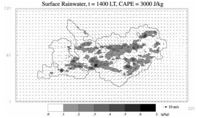
FIG. 14. Surface rainwater and vector field at t = 1400 LT for experiment with a CAPE of 3000 J \text{kg}^{-1} .
