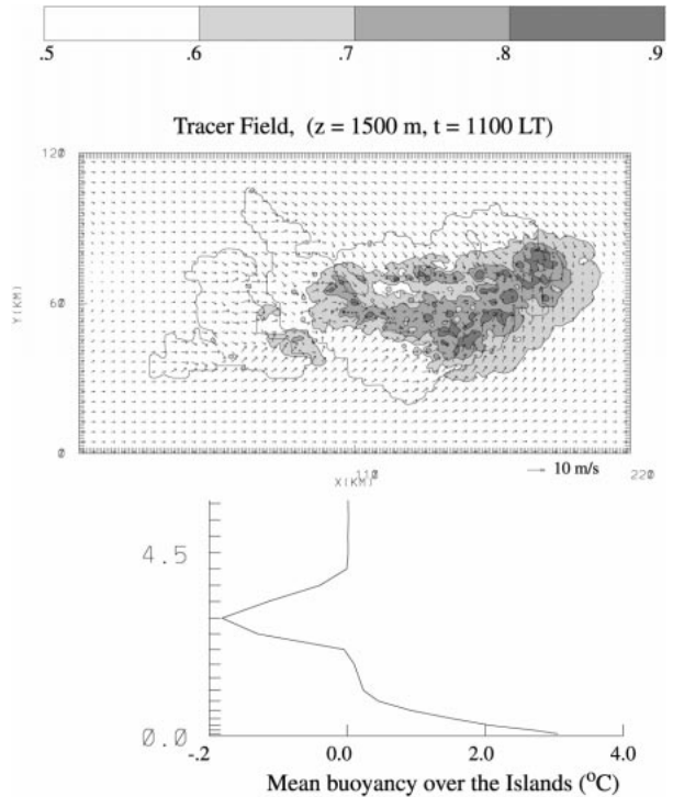
FIG. 5. (a) Concentration of tracer field at z = 1500 m overlaid on surface vector field ( t = 1100 LT). Initially, the tracer field is horizontally homogenous with a value of one at the surface, linearly decreasing to zero at 3 km. (b) Vertical profile of mean buoyancy field above the Tiwi Islands. Note that the scale on the negative side has been expanded by a factor of 10.
