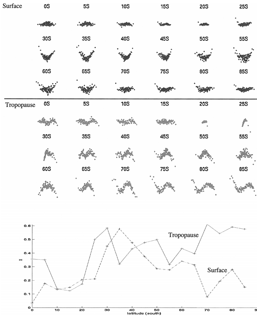
FIG. 4. RDMs are shown for the Southern Hemisphere along 155°E using NCEP–NCAR reanalysis data. Results using barometric pressure (a) at the surface and (b) at the height of the tropopause. (c) Amount of low-dimensional nonlinearity identified by the RDM (using a statistic defined in the paper) as a function of latitude.
