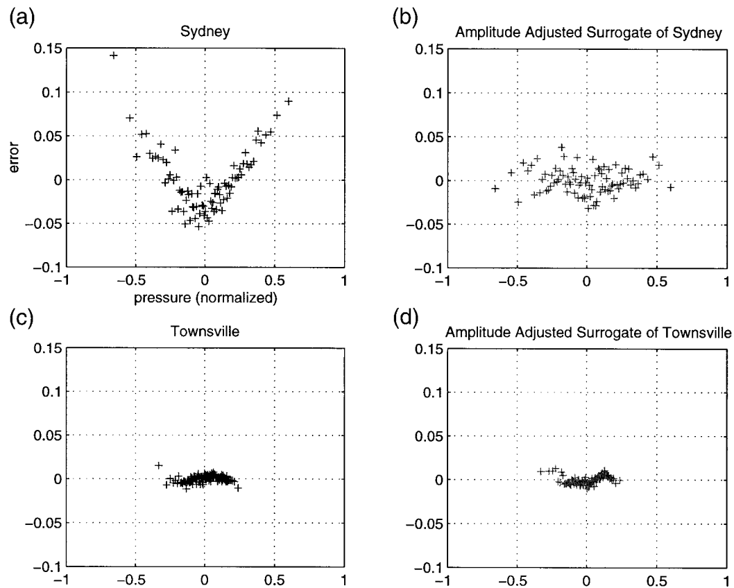
FIG. 1. (a), (c) RDMs using a short-term linear predictive model [Eq. (1)] of daily averaged observed surface pressure (spanning 37 yr) for Sydney (33.52°S, 151.13°E) and Townsville (19.16°S, 146.48°E), Australia (see section 3 for details of the RDMs are computed). (b), (d) RDMs of the corresponding RDMs from amplitude adjusted surrogates (similar, but consistent with a linear signal hypothesis; detailed in section 3a) of the respective time series. Note the destruction of the structure between (a) and (b).
