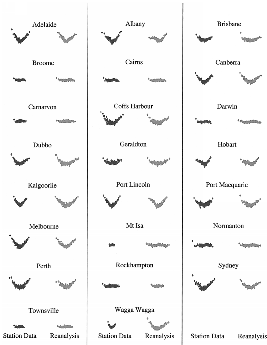
FIG. 3. RDMs for 23 sites on the Australian continent using daily averaged observed surface pressure spanning 37 yr are shown on the left. On the right are the corresponding RDMs from reanalysis data. Note the good agreement at most of the stations, which is in contrast to the results of Sugihara et al. (1996).
