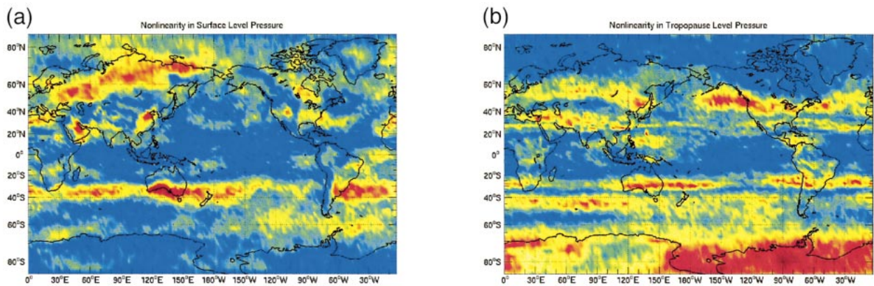
FIG. 5. RDMs were calculated using 39 yr (1957–96) of daily averaged surface pressure from NCEP–NCAR reanalysis data (a) at the surface and (b) at tropopause height. A statistic (detailed in section 3b) was then applied to each RDM to measure the amount of low-dimensional nonlinearity (structure). Red regions indicate RDMs with coherent structure.
