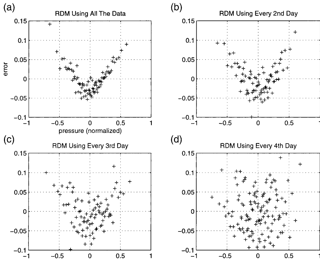
FIG. 2. RDMs are calculated on daily averaged observed surface pressure (spanning 37 yr) for Sydney (33.52°S, 151.13°E), Australia, at different sampling rates from every day to every fourth day. Note the break down in structure as the sampling rate decreases.
