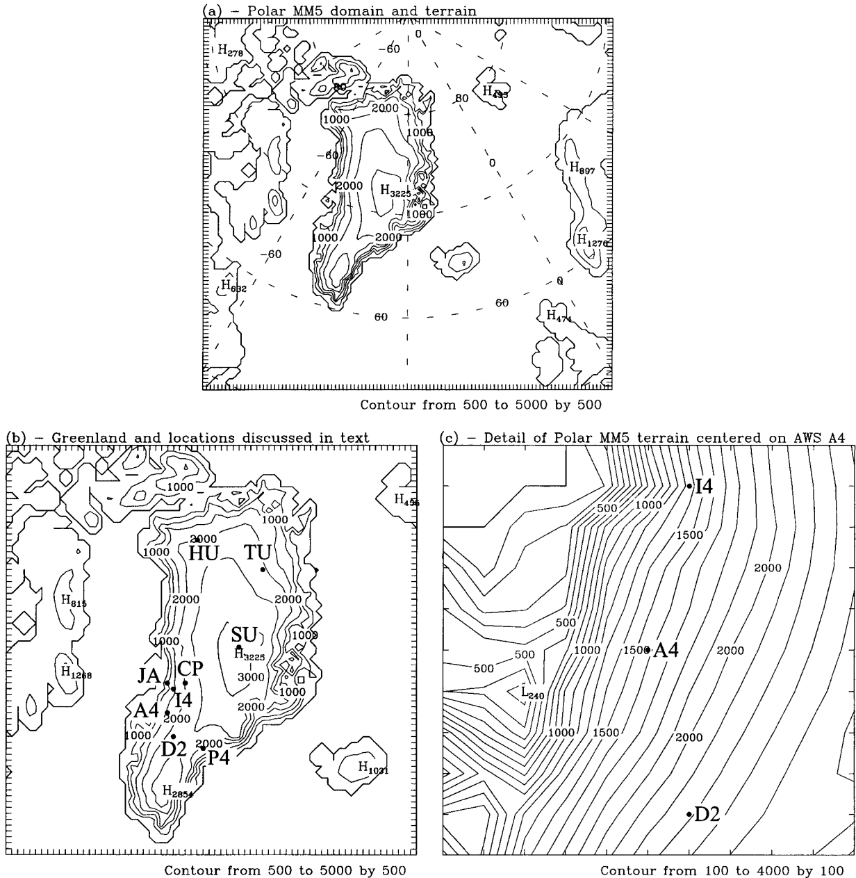
FIG. 1. (a) Map of Polar MM5 model domain, with terrain elevation contours (solid lines, 500-m contour interval), zero elevation contour (bold line), and latitude (dashed lines, 10° contour interval) and longitude (dashed lines, 30° contour interval); (b) detail of Polar MM5 model domain centered on Greenland, with terrain elevation contours (solid lines, 500-m contour interval), zero elevation contour (bold line), and locations of sites discussed in text marked with filled circles (HU: Humboldt AWS, TU: Tunu-N AWS, SU: Summit AWS, JA: JAR 1 AWS, CP: Crawford Point AWS, A4: KABEG AWS A4, D2: Dye-2 AWS, and I4 and P4: location of aircraft profiles); and (c) detail of Polar MM5 model domain centered on KABEG AWS A4, with terrain elevation contours (solid lines, 100-m contour interval), zero elevation contour (bold line), and location of sites I4, A4, and D2 marked with filled circles. Tick marks on borders of each panel indicate spacing of model grid points (40 km).
