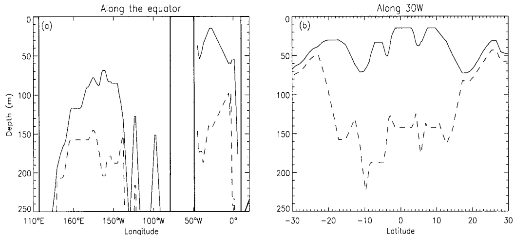
FIG. 7. Minimum vertical displacement that would destabilize the water column (solid line) and depth of the corresponding level (dashed line) along the (a) equatorial section and (b) Atlantic meridional section at 30°W.
