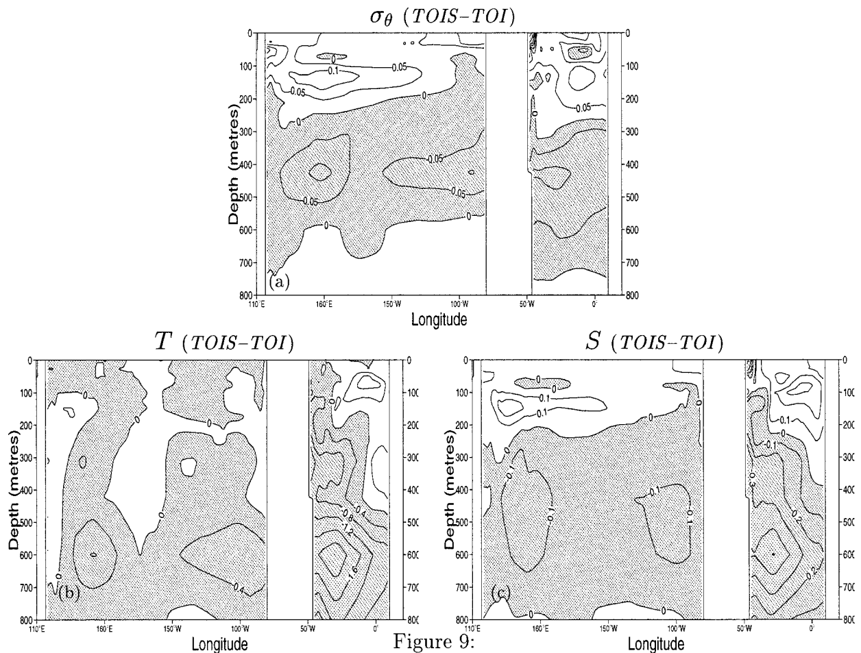
FIG. 9. Equatorial section of the difference TOIS - TOI for the 6-yr mean (1993-98) for (a) \sigma_\theta , (b) temperature, and (c) salinity. Negative values are shaded.
