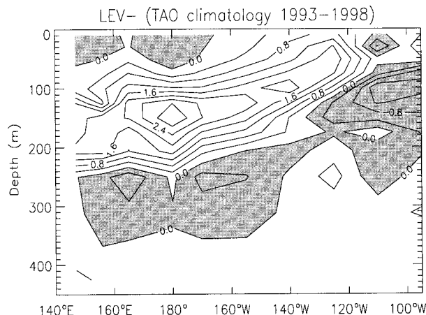
FIG. 4. Equatorial section of temperature. Difference between the annual mean Levitus climatology and the 1993–98 TAO climatology. Negative values are shaded. Contour interval is 0.4^{\circ}\text{C} .
