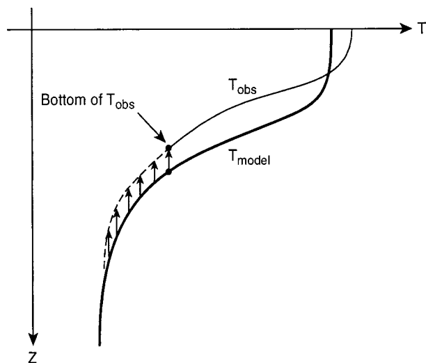
FIG. 1. Schematic of the vertical displacement (first part of the TH99 scheme). The displacement is the difference between the depth of the deepest observed (or, as in our case, the output of the OI) temperature (thin solid line) and the depth of the same temperature in the model profile (bold solid line). This displacement is then used to lift (as in the figure) or lower the model profile in order to complete the observed profile below the deepest observed T (dashed line).
