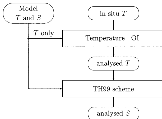
FIG. 2. Schematic of the data assimilation system. TH99 scheme is the salinity scheme.
