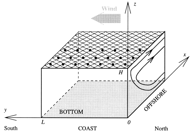
FIG. 1. Model setup. Bullets at the surface show locations of the observations used in the computations.
