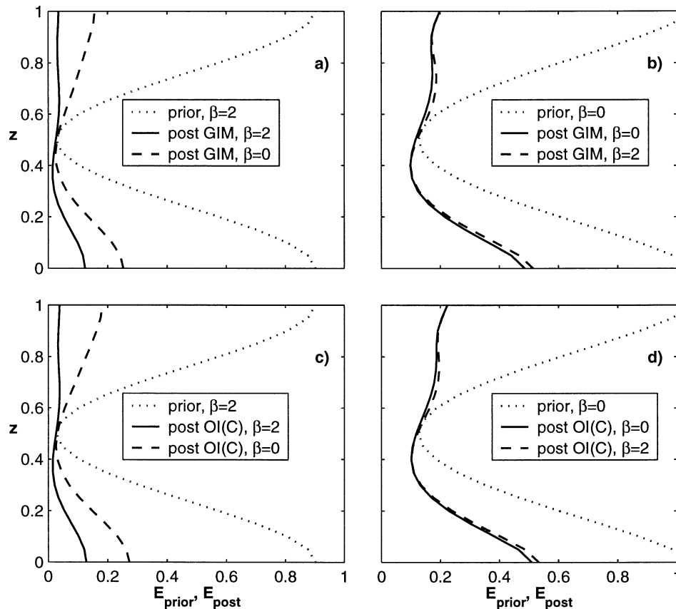
FIG. 9. Effect of misspecification of the model error covariance in the vertical: prior and posterior variance are shown as functions of z at x = 0.2 , y = 1 , t = 70 . w_m = 0.2/\pi^\beta , w_c = \infty , w_d = 1 , L_y = 0.5 . A legend for each plot shows the value of the smoothing parameter \beta : the number next to curve prior is the "true" statistical parameter for all the curves on the plot; the numbers next to curves "post" (posterior variance) are our statistical hypothesis, correct or incorrect: (a), (b) GIM; (c), (d) OI.
