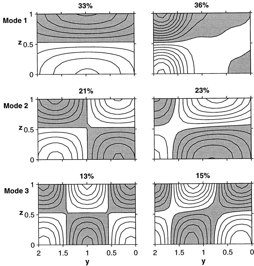
FIG. 7. First singular vectors of \mathbf{P}_{TT}\mathbf{H}' (left panels) and \mathbf{C}_T\mathbf{H}' (right panels) shown in the alongshore section x = 0.15 ; shaded area is for the positive values, contour offset is 0.01. L_y = 0.5 , w_m = 0.2 , w_c = \infty , w_d = 100 . Percent numbers indicate how much variability is explained by the mode.
