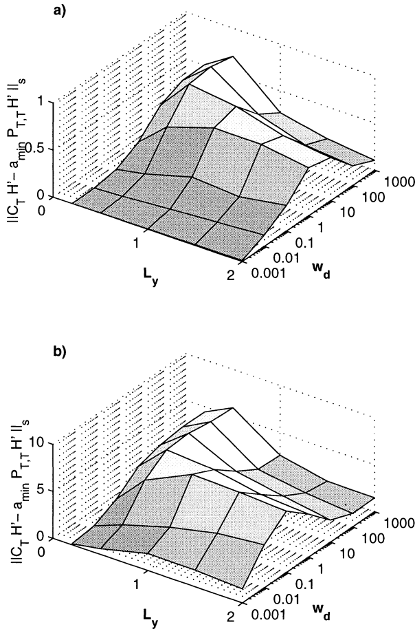
FIG. 5. Norm (46) of \mathbf{C}_T \mathbf{H}' - a_{\min} \mathbf{P}_{T,T} \mathbf{H}' as a function of L_y and w_d : (a) w_m = \infty, w_c = 10 ; (b) w_m = 0.2, w_c = \infty .
