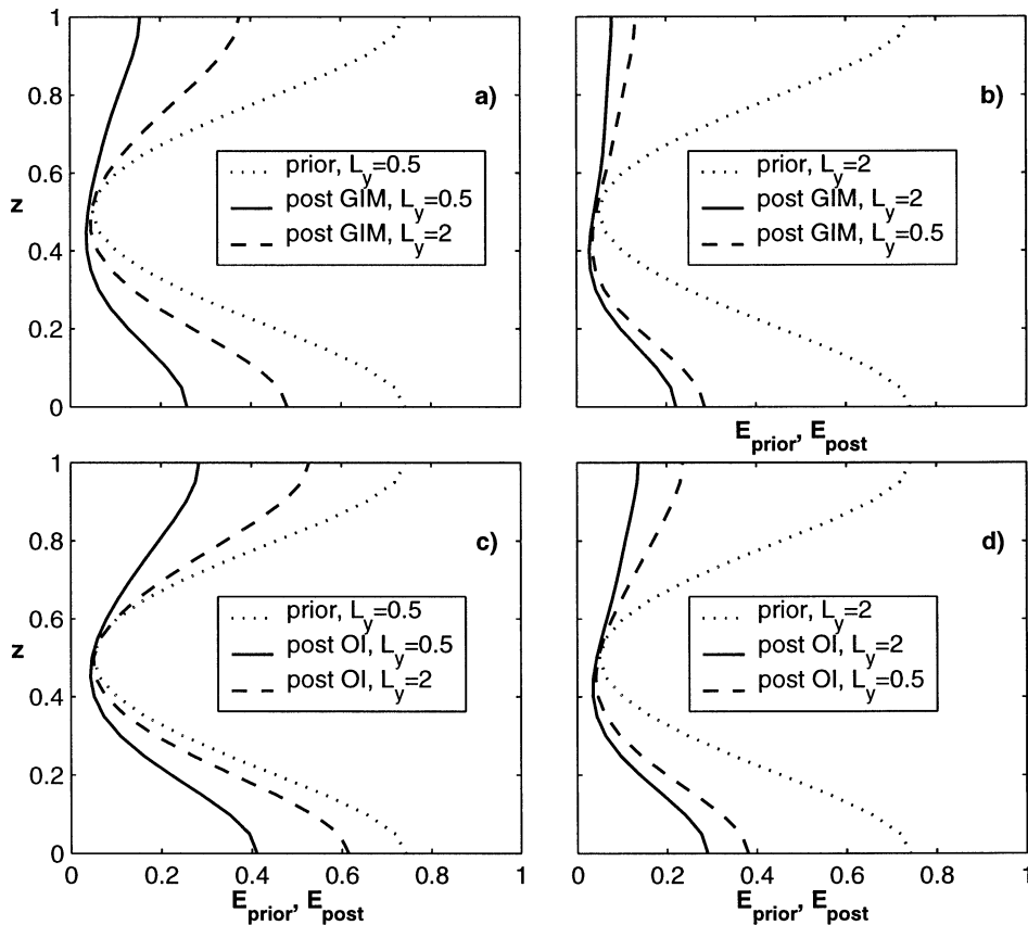
FIG. 10. Effect of over- or underestimation of the error decorrelation length scale for the wind stress: prior and posterior variance are shown as functions of z at x = 0.2, y = 2, t = 70 . w_m = \infty, w_c = 1, w_d = 1 . A legend for each plot shows the value of the smoothing parameter L_y : the number next to curve prior is the true statistical parameter for all the curves on the plot; the numbers next to curves post (posterior variance) are our statistical hypothesis, correct or incorrect: (a), (b) GIM; (c), (d) OI.
