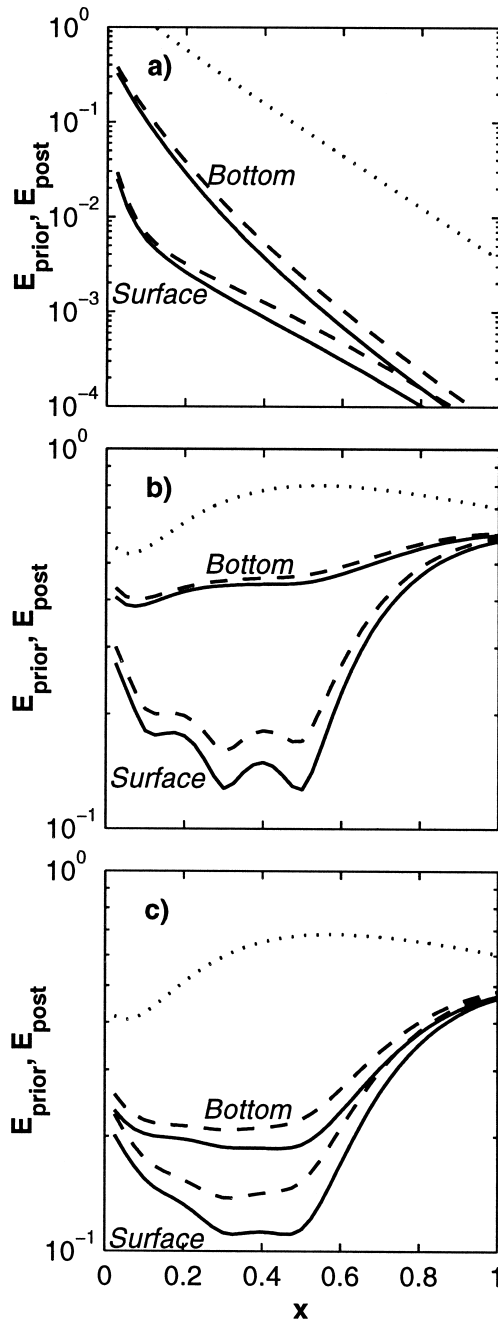
FIG. 4. Variance of the GIM- and KF-derived solutions vs x at the points, y = 1 , t = 40 , surface and bottom. Legend is the same as in Fig. 3. (a) Case c + IB, w_m = w_{IPV} = \infty , w_c = 10 , w_{IB} = 0.084 , w_d = 100 ; (b) case m + IPV, \beta = 0 , w_m = 0.2 , w_{IPV} = 0.017 , w_c = w_{IB} = \infty , w_d = 1 ; (c) case m + IPV, \beta = 2 , w_m = 0.2/\pi^\beta , w_{IPV} = 0.017/\pi^\beta , w_c = w_{IB} = \infty , w_d = 1 .
