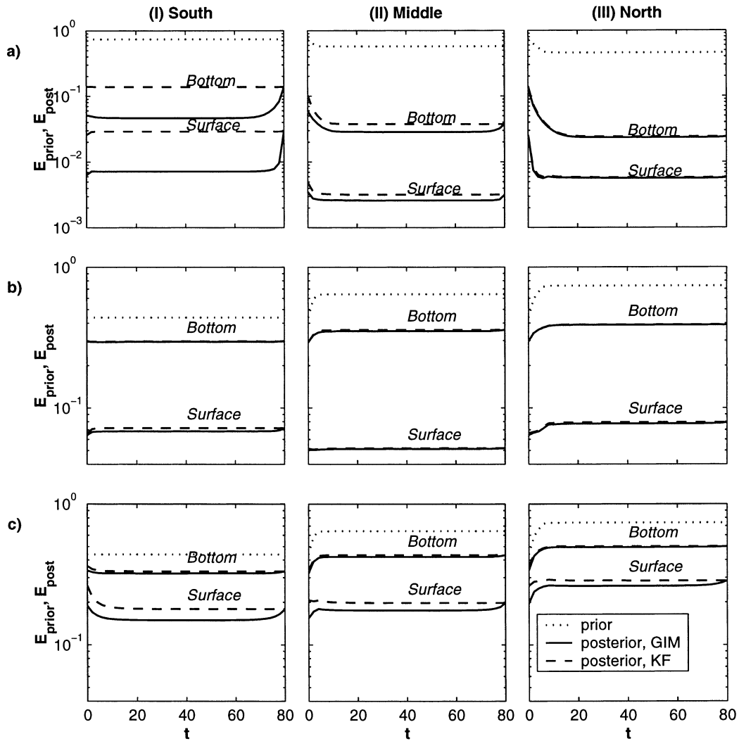
FIG. 3. Prior and posterior variance of the GIM- and KF-derived solutions vs time at six different points, all at the offshore distance x = 0.2 . Columns: (I) south ( y = L = 2 ), (II) middle ( y = 1 ), and (III) north ( y = 0 ). Weights (a) w_m = w_{IPV} = \infty , w_c = 10 , w_{IB} = 0.084 , w_d = 100 ; (b) w_m = 0.2 , w_{IPV} = 0.017 , w_c = w_{IB} = \infty , w_d = 100 , \beta = 0 ; (c) the same as in (b) but with the lower data weight w_d = 1 .
