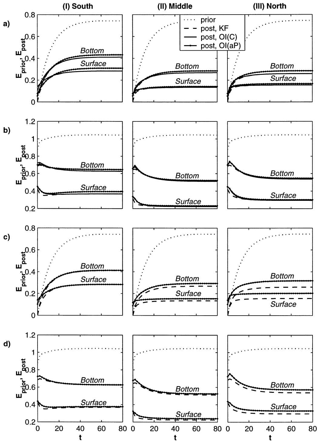
FIG. 8. Variance of OI- and KF- derived solutions vs time at six different points at x = 0.2, L_y = 0.5 . Columns: (I) south ( y = L = 2 ), (II) middle ( y = 1 ), and (III) north ( y = 0 ). Rows: (a) w_m = w_{IPV} = \infty, w_c = 1, w_d = 1, a = a_{min} = 0.5 ; (b) w_m = 0.2, w_{IPV} = 0.017, w_c = \infty, w_d = 1, a = a_{min} = 0.45 ; (c) and (d) are the same as in (a) and (b), correspondingly, but with a = 1 .
