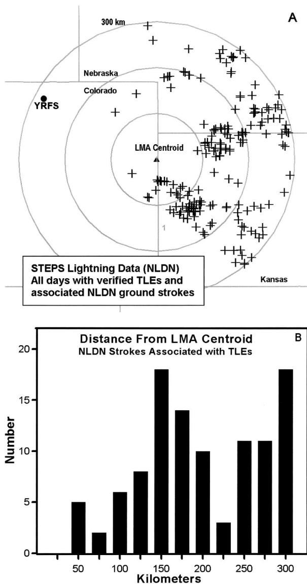
FIG. 1. (a) NLDN-determined locations of SP+CGs observed during the STEPS campaign and (b) their distribution as a function of range (km) from the centroid of the LMA. LLTV cameras monitored sprites optically from their location at YRFS.
