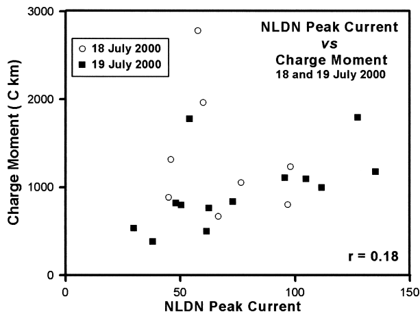
FIG. 5. NLDN peak current vs charge moment change computed by the MIT technique for SP+CGs for MCSs near the LMA on 18–19 Jul 2000. The computed value of R is 0.18.
