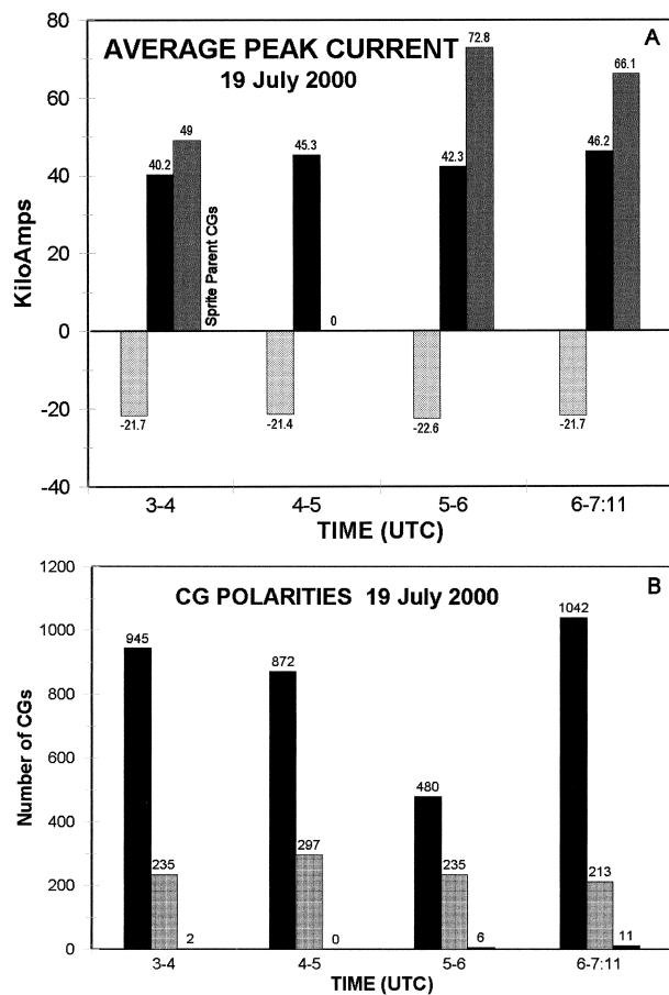
FIG. 3. (a) Hourly average peak currents (kA) for NLDN-detected strokes from both MCSs, for -CGs, +CGs (black), and SP+CGs (gray). (b) Number of NLDN-detected -CGs (black), +CGs (stippled), and SP+CGs during the sprite observation period 0300–0711 UTC 19 Jul 2000.
