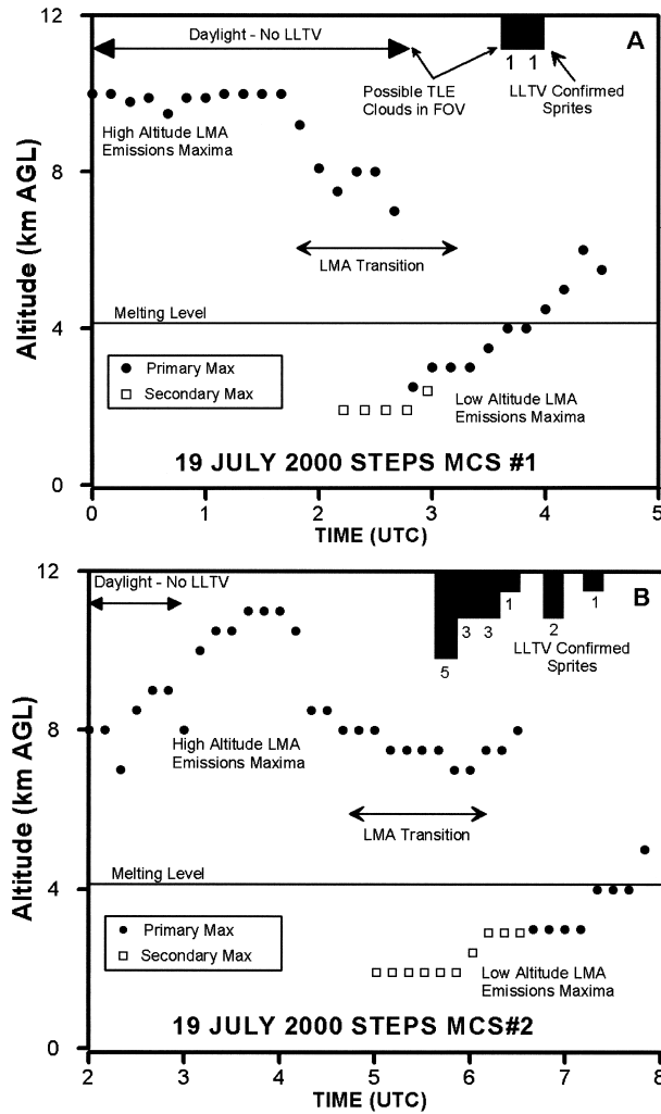
FIG. 6. (a) History of the altitude of the centroid of max VHF emissions detected by the LMA for MCS 1 on 19 Jul 2000 as it moved through the STEPS domain. The occurrence of sprites is indicated at the upper right. (b) The same as (a), but for MCS 2.
