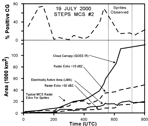
FIG. 4. History of key parameters for MCS 2 on 19 Jul 2000. The percentage of strokes with positive polarity detected by the NLDN is shown on top. Also shown are the area covered by VHF electrical emissions detected by the LMA, the area of base radar reflectivities >10 and >30 dBZ, and the area of the cloud canopy on the GOES-8 infrared imagery. The period during which 15 sprites were detected from 0551 to 0711 UTC is indicated.
