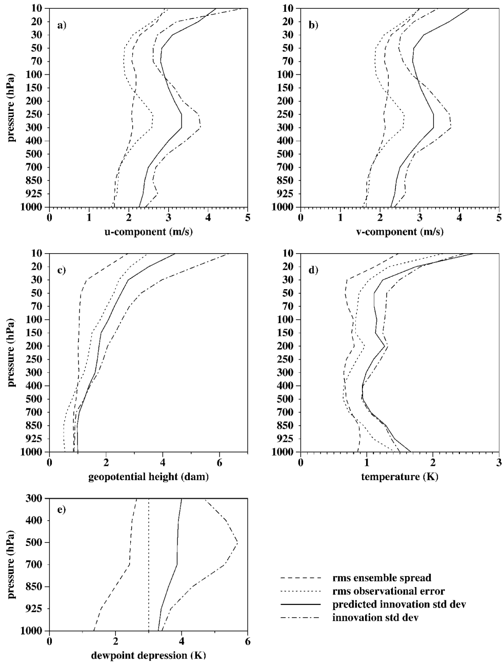
FIG. 5. Comparison of error amplitudes that have been averaged over a 10-day experimental period. Shown are the predicted innovation std dev (solid) that should match the observed innovation std dev (dashed-dotted). The predicted std dev is computed from the rms observational error (dotted) and the rms ensemble spread (dashed).
