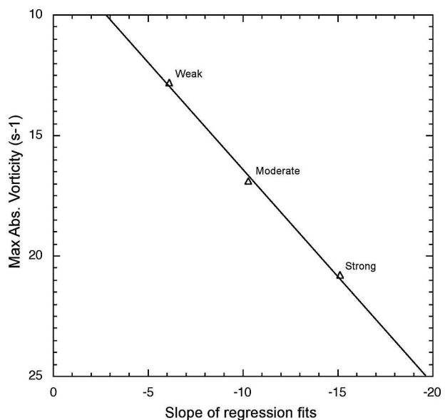
FIG. 4. The maximum absolute vorticities ( \text{s}^{-1} , averaged for each bin) plotted against the corresponding slope of the linear regressions seen in Fig. 3.
