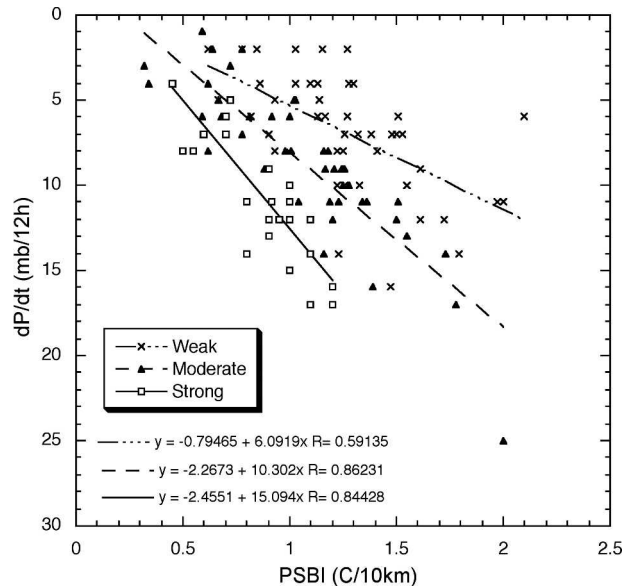
FIG. 3. The ASCII dataset (1991–2002) of ETC [\Delta P (12 \text{ h})^{-1}] vs PSBI broken down into bins of 500-mb vorticity ( 10^{-5} \text{ s}^{-1} ).
