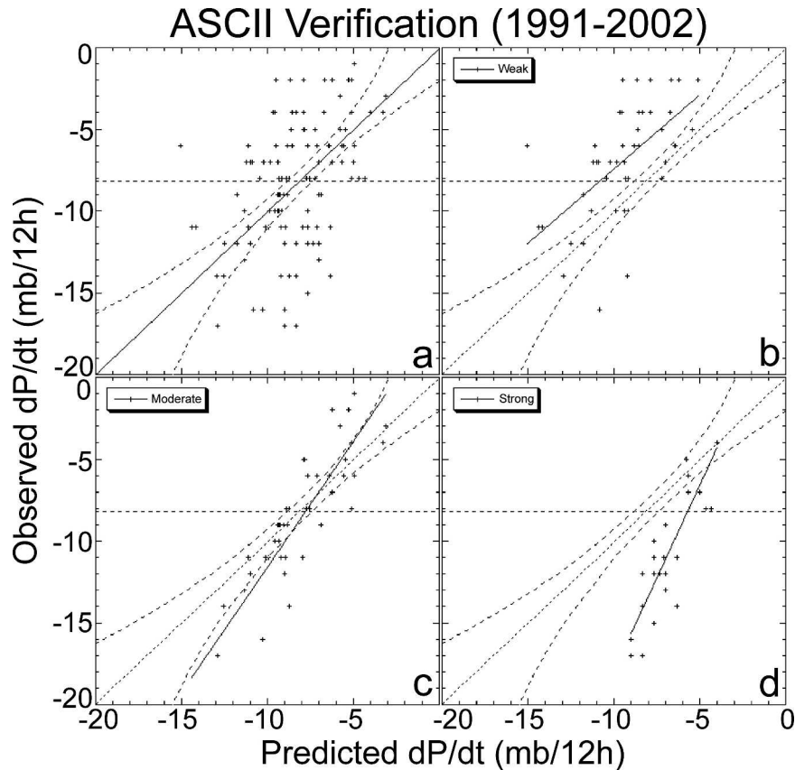
FIG. 5. The observed deepening rate [ \text{mb} (12 \text{ h})^{-1} ] of cases from the 1991–2002 dataset plotted against the predicted deepening rate [ \text{mb} (12 \text{ h})^{-1} ] from the updated ASCII regression equation seen in Fig. 2. The center line shows a perfect correlation bound on both sides by a 95% confidence interval calculated for the entire dataset. The horizontal line marks the mean deepening rate for the entire dataset. (a) The full distribution, as well as (b) the weakly forced, (c) moderately forced, and (d) strongly forced bins are shown.
