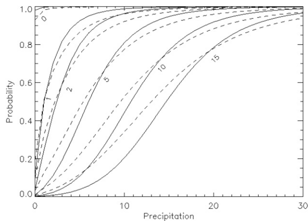
FIG. 4. Probability distribution [ \Pr(A \leq q) ] based on the extended logistic regressions (EPS-FULL) for the Ourthe during winter at forecast days 3 (solid line) and 6 (dashed line). (left to right) The curves correspond to ensemble averages of 0, 1, 2, 5, 10, and 15 \text{mm day}^{-1} .
