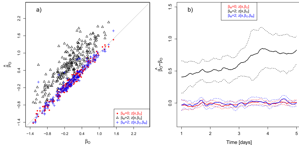
FIG. 1. (a) Estimated observation bias as a function of specified bias and (b) time series of estimated observation bias minus assigned bias. In (b) the mean (solid lines) and standard deviation (dashed lines) of the 240 observing locations are shown. Colors distinguish different experiments: a perfect model with \hat{\beta}_O estimated (red), an imperfect model with \hat{\beta}_O estimated (black), and an imperfect model with both \hat{\beta}_M and \hat{\beta}_O estimated (blue).
