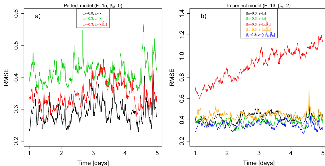
FIG. 2. Time series of prior RMSE for different experiments (colors) using (a) a perfect model with and without spatially constant observation bias of \beta_O = 0.3 , and (b) an imperfect model with \beta_M = 2 . Legends show specified observation biases and the augmented vector estimated in the assimilation.
