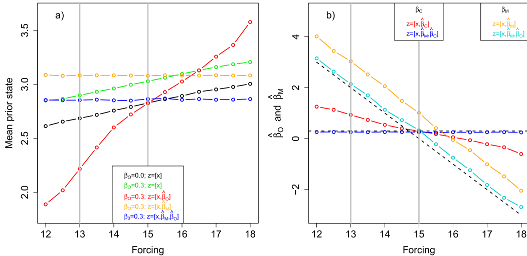
FIG. 5. (a) The prior mean state and (b) the estimated parameter values vs the forcing term F in the assimilating model. The legend in (a) shows the specified observation bias and the augmented vector estimated in the assimilation. In (b) the specified biases are shown in dashed black lines. The vertical gray lines show, for reference, the forcing values for the perfect and imperfect models used in the estimation experiments reported in prior figures.
