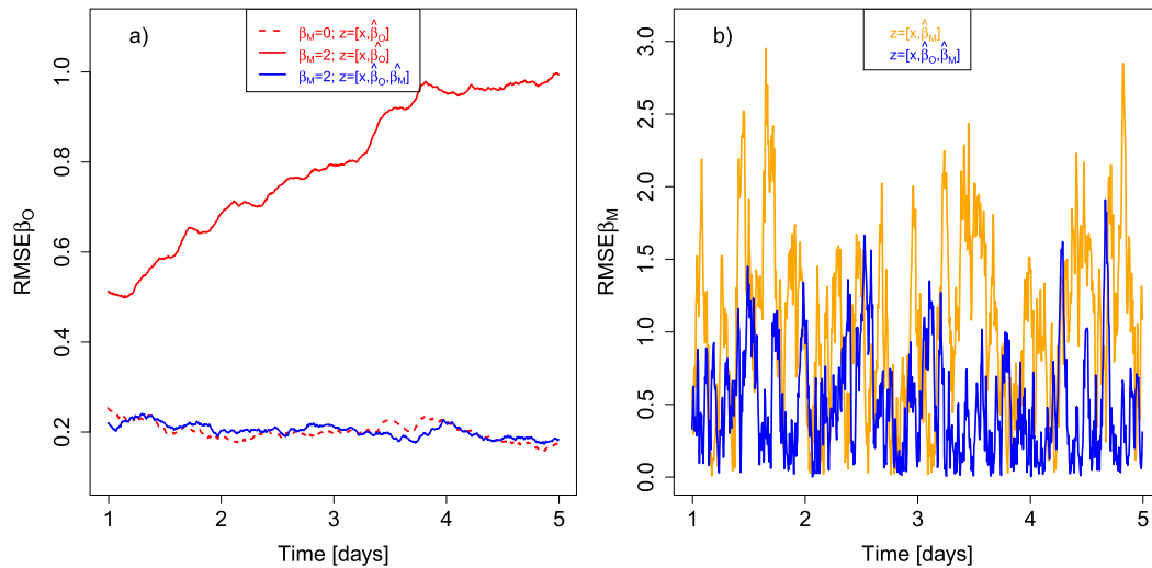
FIG. 3. Time series of (a) RMSE \beta_O and (b) RMSE \beta_M for different parameter estimation experiments. The legend in (a) shows the model forcing bias and the augmented vector estimated in the assimilation. In (b) the model forcing bias is \beta_M = 2 .
