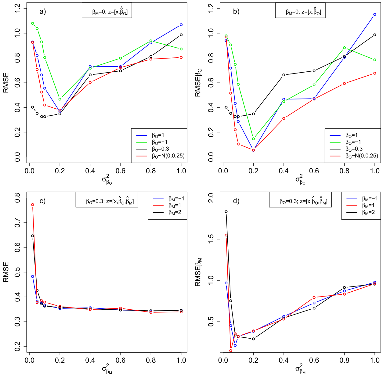
FIG. 6. Perfect-model results for (a) RMSE and (b) RMSE \beta_O as a function of \sigma_{\beta_O}^2 . Colors indicate specified observation bias ( \beta_O ), with \beta_O estimated in the assimilation. Imperfect-model results for (c) RMSE and (d) RMSE \beta_M as function of \sigma_{\beta_M}^2 . Colors indicate specified forcing bias ( \beta_M ), with both \beta_O and \beta_M estimated in the assimilation.
