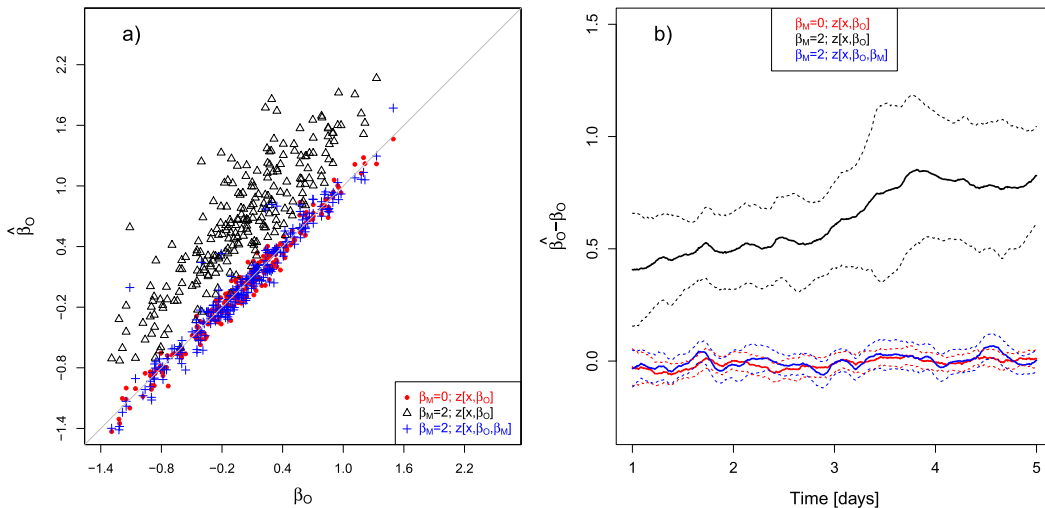
FIG. 1. (a) Estimated observation bias as a function of specified bias and (b) time series of estimated observation bias minus assigned bias. In (b) the mean (solid lines) and standard deviation (dashed lines) of the 240 observing locations are shown. Colors distinguish different experiments: a perfect model with \hat{\beta}_O estimated (red), an imperfect model with \hat{\beta}_O estimated (black), and an imperfect model with both \hat{\beta}_M and \hat{\beta}_O estimated (blue).
