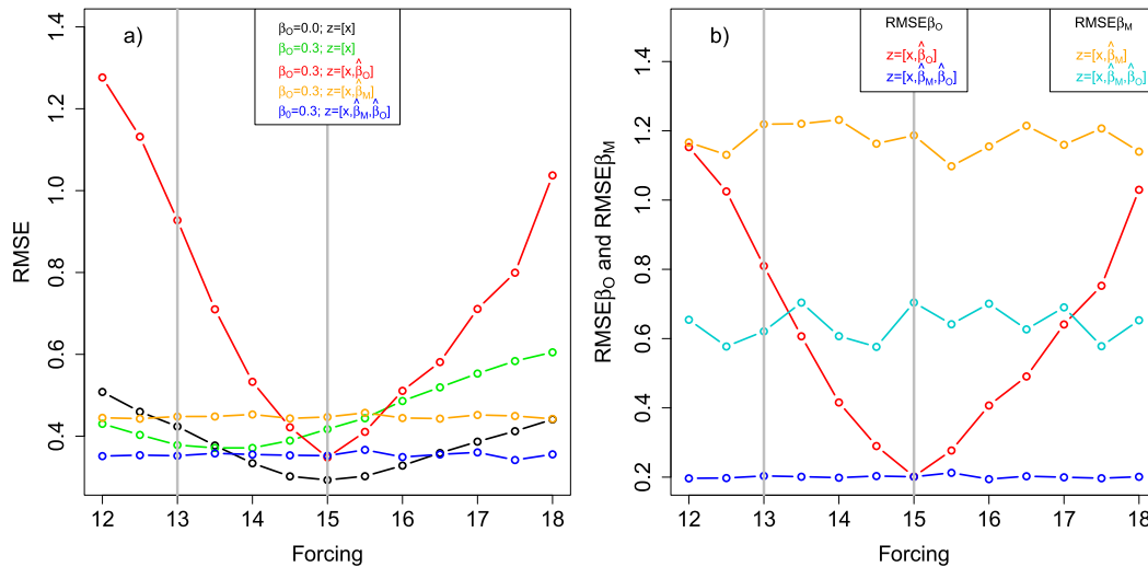
FIG. 4. (a) Prior RMSE, and (b) both RMSE \beta_O and RMSE \beta_M vs the forcing term F in the assimilating model. The legend in (a) shows the specified observation bias and the augmented vector estimated in the assimilation. In (b) the observation bias is \beta_O = 0.3 . The vertical gray lines show, for reference, the forcing values for the perfect and imperfect models used in the estimation experiments reported in prior figures.
