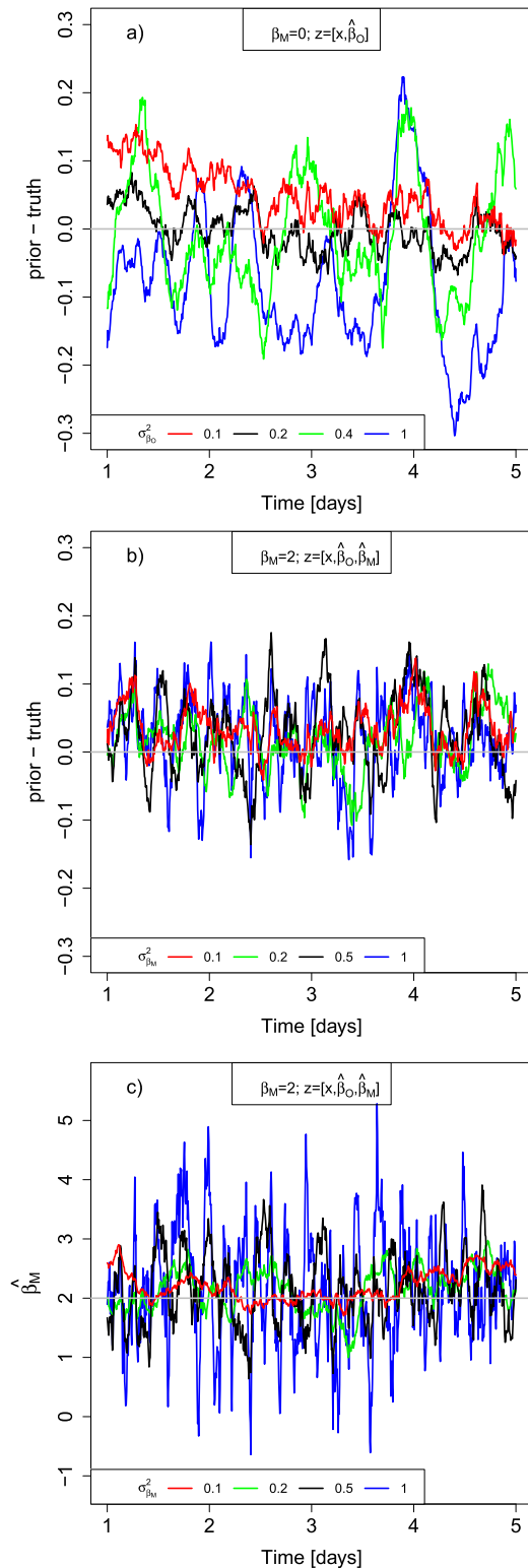
FIG. 7. (a) Perfect-model experiment error time series (prior minus truth) for different minimum enforced \sigma_{\beta_O}^2 (colors) when estimating a assigned observation bias \beta_O = 0.3 . (b) Imperfect-model experiment time series for state errors and (c) \hat{\beta}_M for different minimum enforced \sigma_{\beta_M}^2 (colors) and estimating both model and observation bias as shown in the upper legend.
