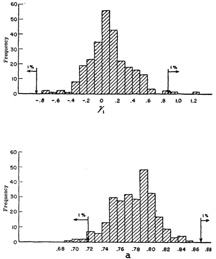
FIGURE 1.—Frequency distributions of \gamma_1 and a , which are measures of skewness and flatness of the distribution of seasonal degree days, computed for 266 weather stations. The vertical arrows prescribe the limits allowed for normality according to Geary and Pearson [2].
