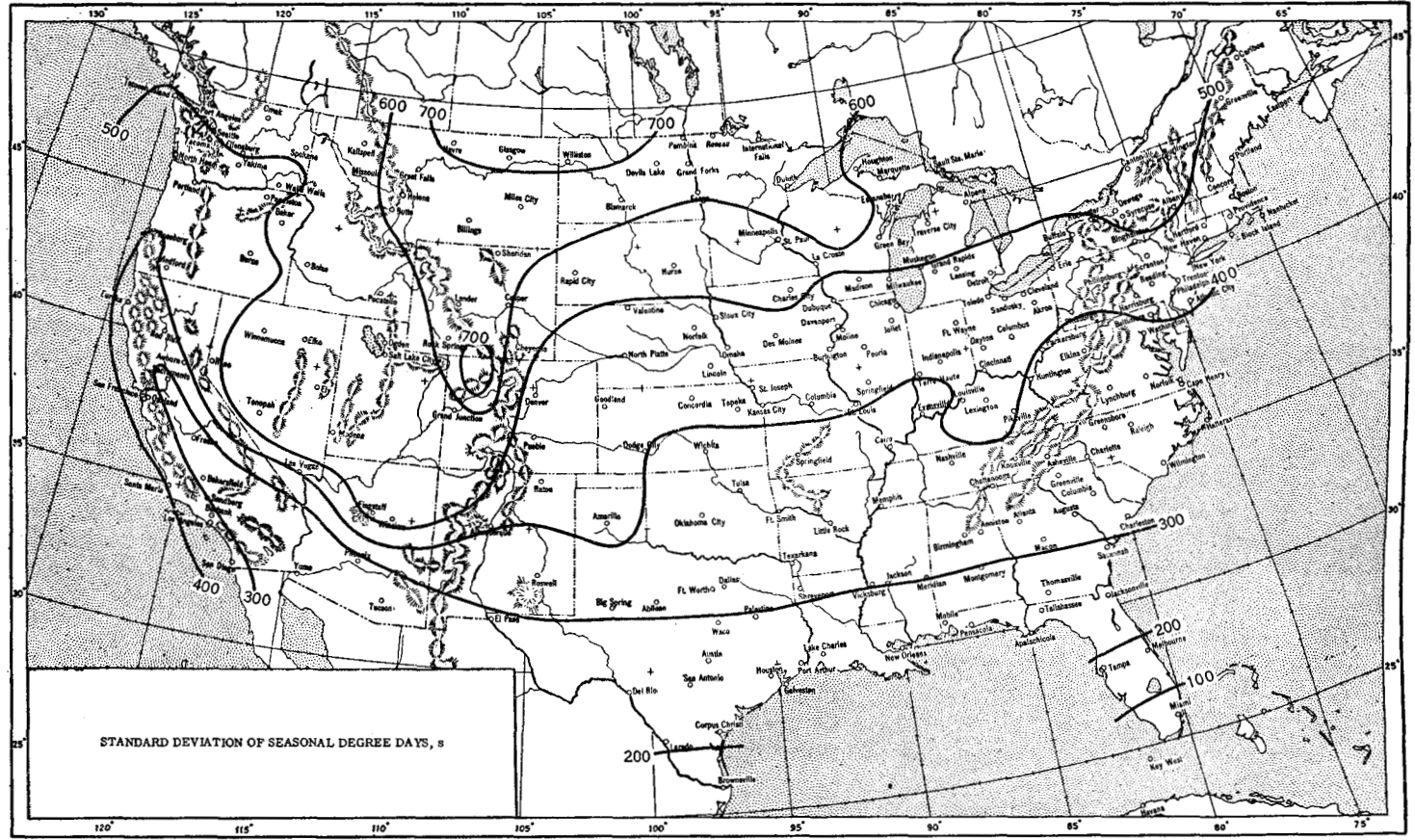
FIGURE 3.—Chart of standard deviation of seasonal heating degree days in the United States, based on data from 266 weather stations. See table 1 for an abbreviated table of the normal probability distribution for use with figures 2 and 3.
