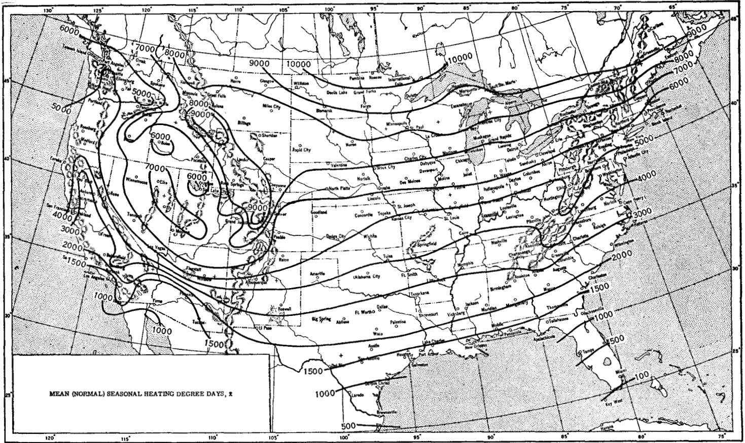
FIGURE 2.—Chart of mean seasonal heating degree days in the United States, based on data from 266 weather stations. Care has been taken to draw the isolines with consideration for local effects of mountains and other topographical features.
