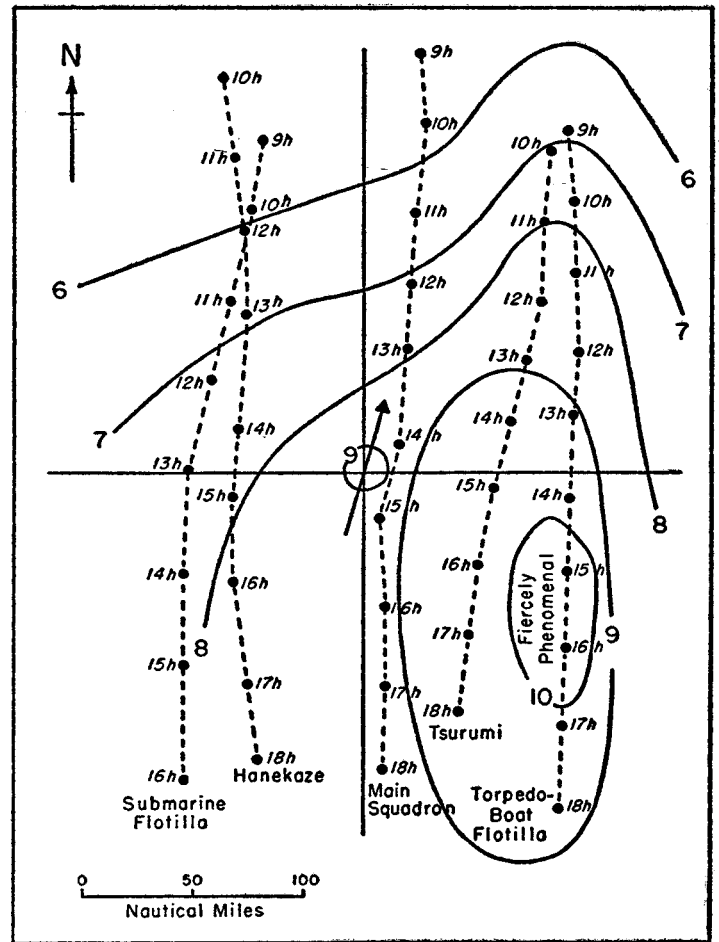
FIGURE 3.—Composite chart showing the state of the sea in the typhoon of September 26, 1935. Intersection of the cross lines represents the center of the typhoon. The arrow through the center indicates the direction of movement of the typhoon. Dots indicate positions of naval units at hourly intervals (JMT). Lines of constant wave heights are drawn for each unit of the sea scale (see scale table in text).
