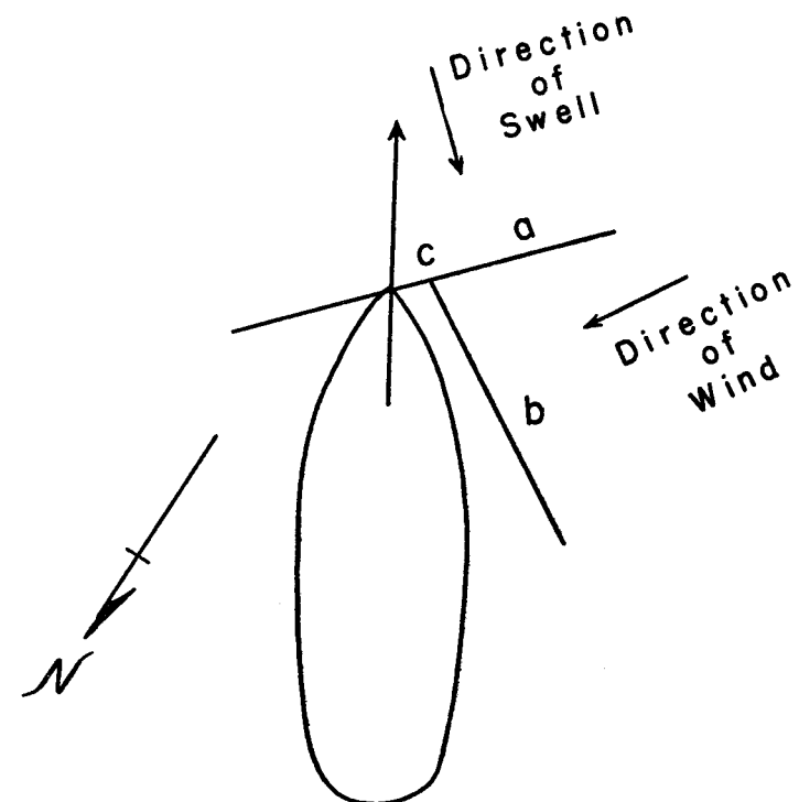
FIGURE 5.—Schematic illustration of the behavior of the sea in the right rear quadrant (1520 JMT) of the typhoon of September 26, 1935. Based on photographs by Lieut. G. Matsuura, looking to the windward on board the cruiser Nachi . The direction of movement of the cruiser was 15 on the 36-point direction scale. a indicates the wave front of swells from the southeast; b , the wave front of wind waves under the influence of wind of speed 27 m. sec. -1 and direction 21; c , pyramidal waves. Note the deviation of the wind to the right of the swell, a marked exception to Tannehill's rule [8].
