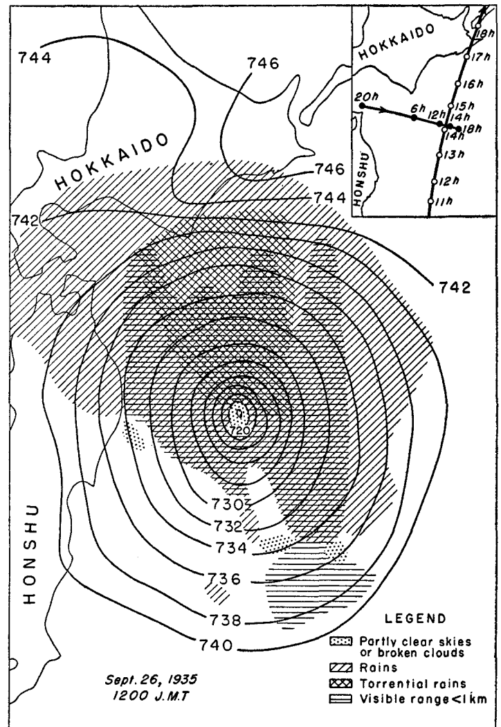
FIGURE 2.—Pressure pattern over the sea to the east of Japan at 1200 JMT, September 26, 1935. Isobars are drawn for each 2 mm. of Hg. (about 2.7 mb.). Shading indicates composite distribution of rains, torrential rains, and poor visibilities (< 1 km.) relative to the center of the typhoon. The inset (upper right) shows the path of the typhoon center during the critical period from 1100 to 1800 JMT, September 26, and the trajectory traversed by the main squadron from 2000 JMT, September 25 to 1800 JMT, September 26.
