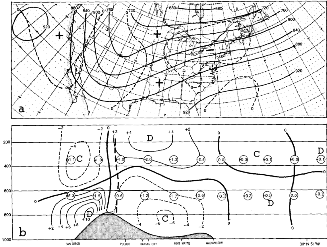
FIGURE 2.—(a) Error in decafeet (dashed lines) of the 12-hr. barotropic forecast from 0000 GMT, January 21, 1959, superimposed on the 500-mb. contours (solid lines) for that time. (b) Cross-section of horizontal divergence in units of 10^{-6} \text{ sec}^{-1} . The numbers in circles are \omega in units of 10^{-3} \text{ mb. sec}^{-1} . Heavy dashed line is the trough line.
