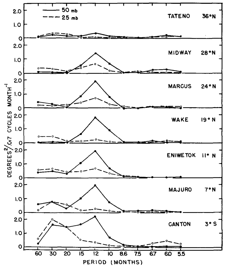
FIGURE 6.—Variance per unit frequency interval of the mean monthly temperature at 50 mb. (solid lines) and 25 mb. (dashed lines) at various latitudes.
