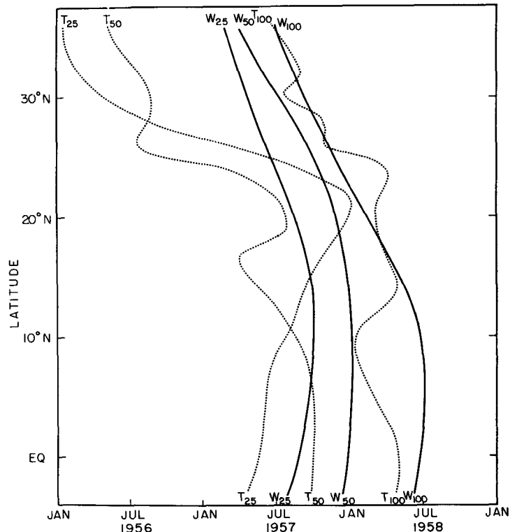
FIGURE 7.—Smoothed time of biennial west wind maxima (solid lines) at 25, 50, and 100 mb. and time of temperature maxima at the three levels (dashed lines) deduced from cross-spectrum analysis of wind and temperature.
