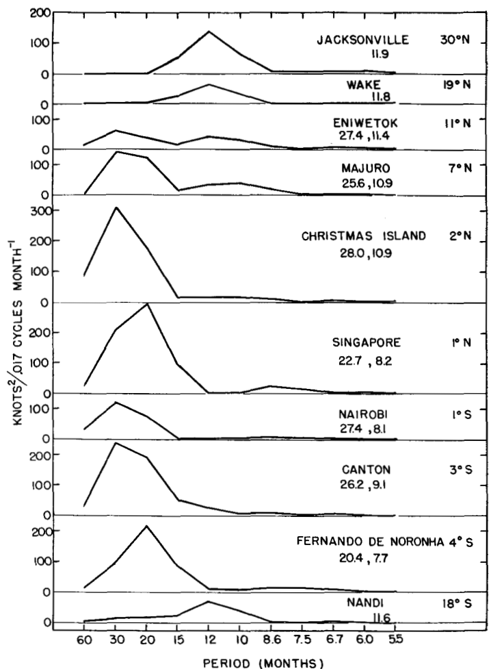
FIGURE 3.—Variance per unit frequency interval of the mean monthly zonal wind component at 50 mb. at selected stations varying in latitude and longitude. The numerals indicate the number of months at which the variance is a maximum, obtained using a weighting technique (see text).
