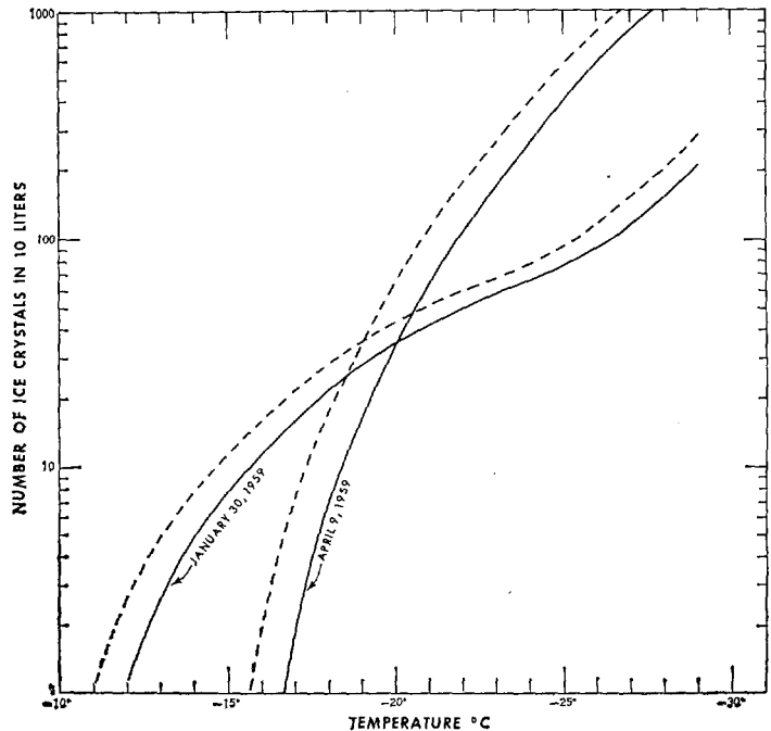
FIGURE 2.—An illustration of the variable consequences of a 1^{\circ}\text{C} . discrepancy in the thermal characteristics between instruments as influenced by differing nuclei spectrum concentrations. The examples are based on two observational series in the Washington, D.C. area selected on the basis of identical indicated concentrations at -20^{\circ}\text{C} . in the original measurements (solid curves) but differing values at other temperatures. Simulated measurements (dashed curves) for an instrument with a thermal discrepancy were obtained by displacing the original measurements 1^{\circ}\text{C} .
