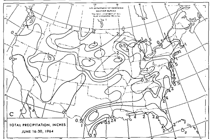
FIGURE 5.—(A) Mean 700-mb. height and departure from normal (both in tens of feet); (B) Departure of average temperature from normal (°F); and (C) Total precipitation (inches) for June 16-30, 1964.
