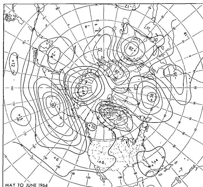
FIGURE 1.—Change of mean 700-mb. height anomaly from May to June 1964, drawn at intervals of 100 ft. with centers in tens of feet and zero isopleth heavy.
