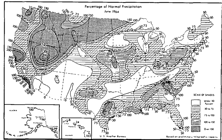
FIGURE 7.—Percentage of normal precipitation for June 1964 (from [2]).
