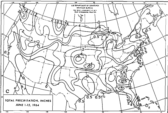
FIGURE 4.—(A) Mean 700-mb. height and departure from normal (both in tens of feet); (B) Departure of average temperature from normal (°F); and (C) Total precipitation (inches) for June 1-15, 1964.
