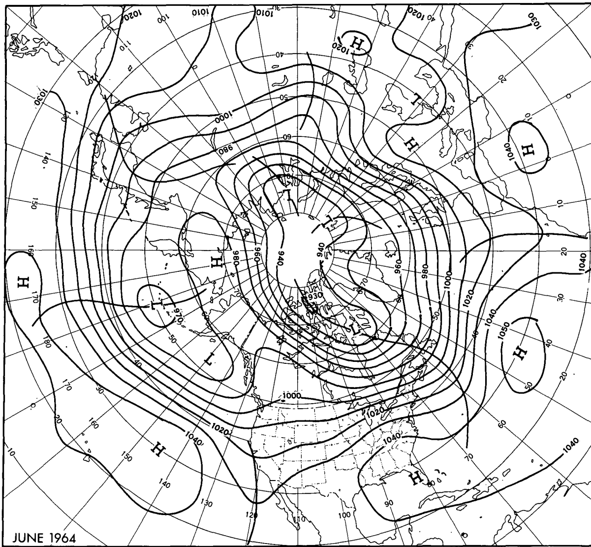
FIGURE 2.—Mean 700-mb. contours (tens of feet) drawn at intervals of 100 ft. for June 1964.
