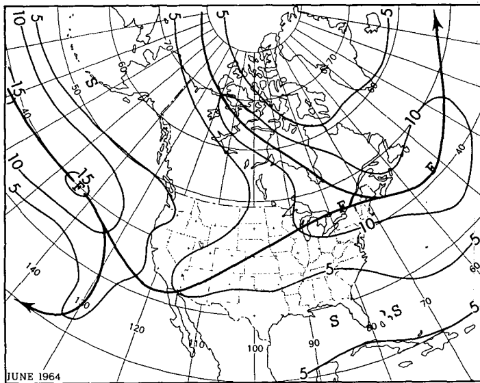
FIGURE 8.—Mean isotachs (meters per second) at 700 mb. for June 1964. Heavy solid arrows indicate principal axes of maximum wind speed.
