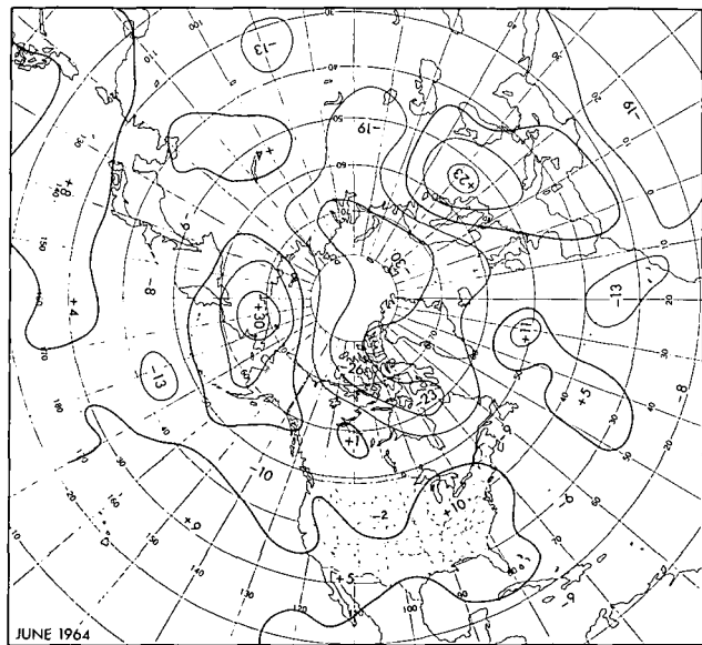
FIGURE 3.—Mean 700-mb. height departures from normal for June 1964 drawn at intervals of 100 ft. with centers in tens of feet and zero isopleth heavy.
