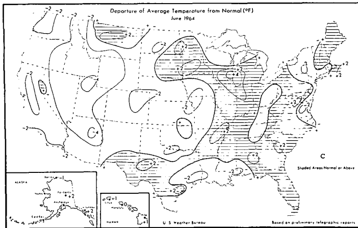
FIGURE 6.—Departure of average surface temperature from normal ( ^{\circ} F) for June 1964 (from [2]).
