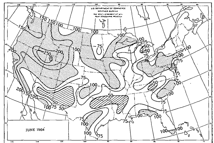
FIGURE 9.—Percentage of normal number of days with 0.01 inch or more precipitation for June 1964.
