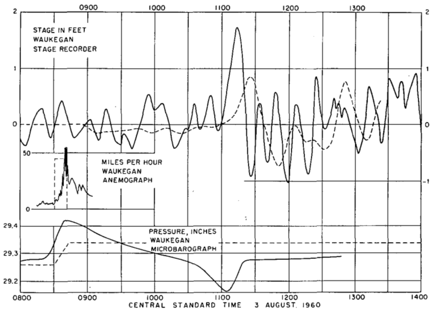
FIGURE 5.—Lake-level, wind, and atmospheric-pressure records at Waukegan, August 3, 1960. The broken curves are for the numerical computation 54 kt., 115° (see section 4).
