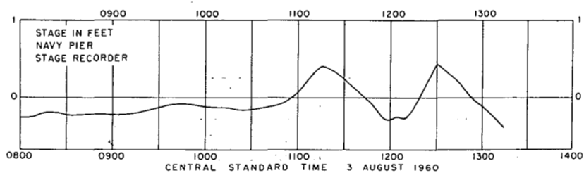
FIGURE 6.—Lake-level records at Calumet Harbor and at Navy Pier, August 3, 1960.
