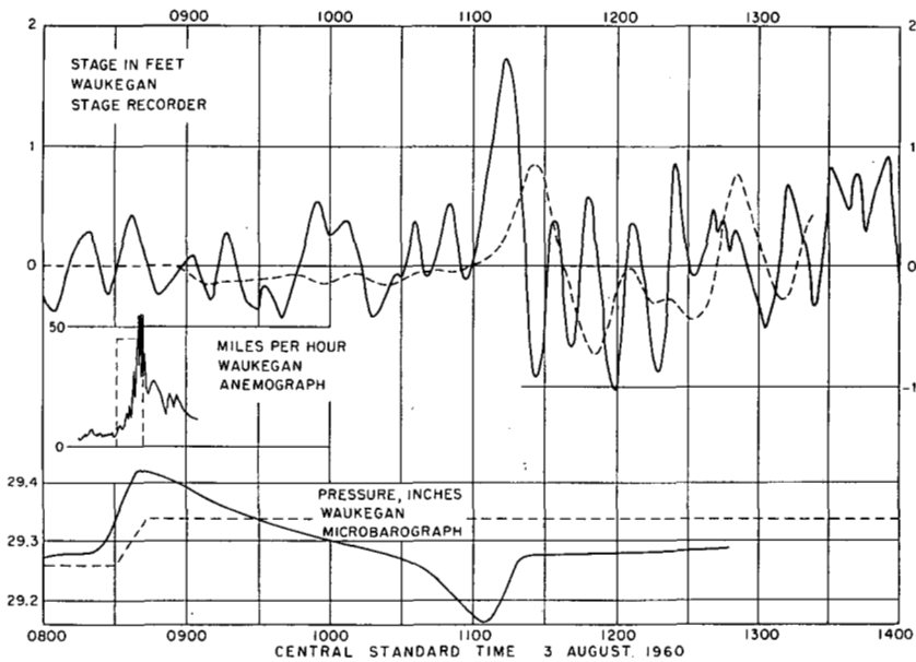
FIGURE 5.—Lake-level, wind, and atmospheric-pressure records at Waukegan, August 3, 1960. The broken curves are for the numerical computation 54 kt., 115° (see section 4).
