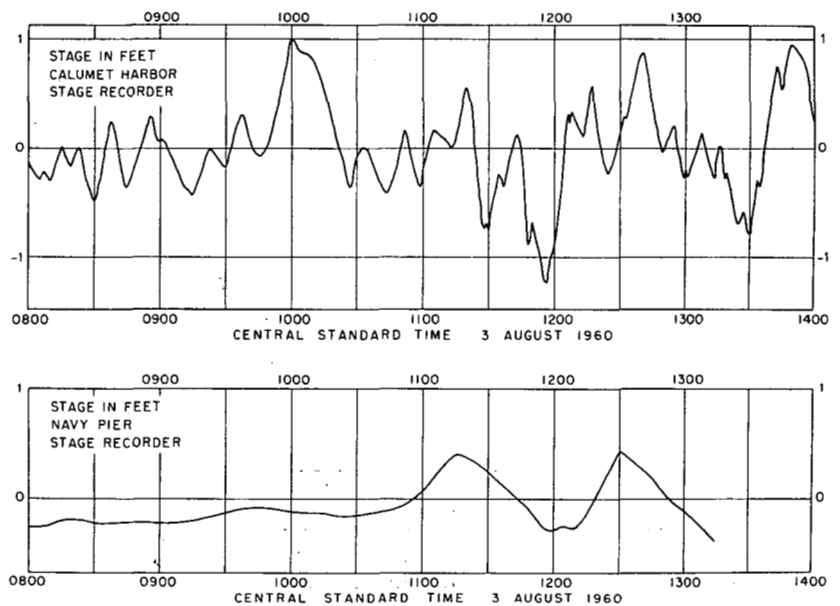
FIGURE 6.—Lake-level records at Calumet Harbor and at Navy Pier, August 3, 1960.
