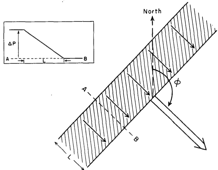
FIGURE 8.—Schematic picture of the hypothetical conditions of pressure and wind which characterize the squall line in the computations by Platzman [6, 7]. The angle \phi defines the direction of motion of the squall line.
