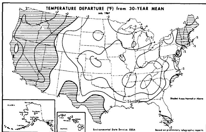
FIGURE 4.—Surface temperature departure from normal (°F.), July 1967 (from [2]).
