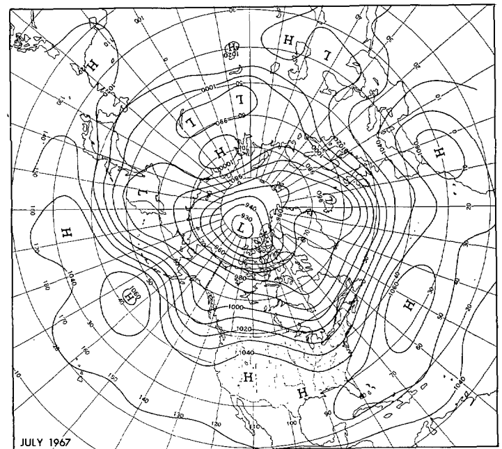
FIGURE 2.—Mean 700-mb. contours (tens of feet), July 1967.
