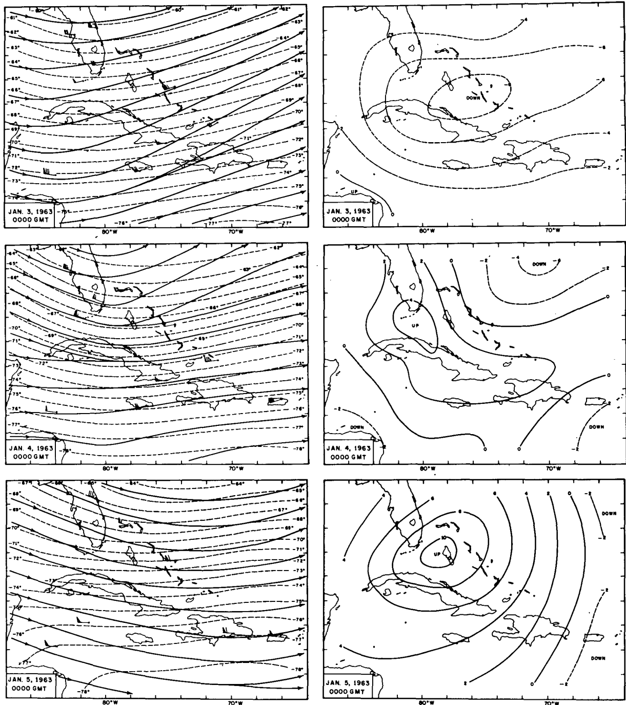
FIGURE 2.—Streamlines and isotherms (left) and vertical motion (right) at 100 mb. at 00 GMT, Jan. 3 to 5, 1963. Wind speeds are indicated in m./sec. (long barb represents 10 m./sec. and short barb 5 m./sec.). Isotherms are shown by dashed lines and labeled in °C. Isopleths of vertical motion are labeled in mm./sec.
