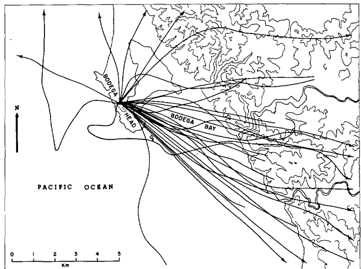
FIGURE 1.—Trajectories of tetroon flights released from Bodega Head, Calif., in September and October 1964. The arrowheads indicate that the tetroon trajectories extend beyond the boundaries of the map. Terrain height is shown at 60-m intervals. The radar was located at the common beginning of the tetroon trajectories.
