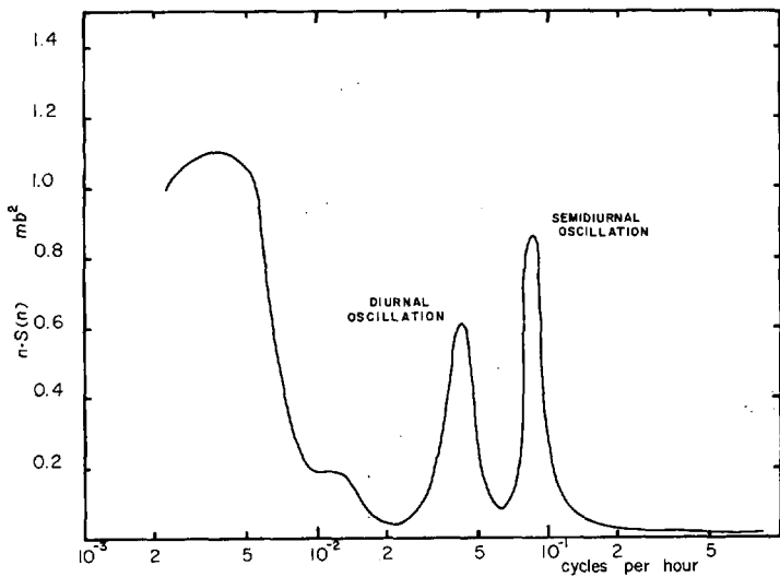
FIGURE 4.—Power spectrum of surface pressure at Palmyra Island.
