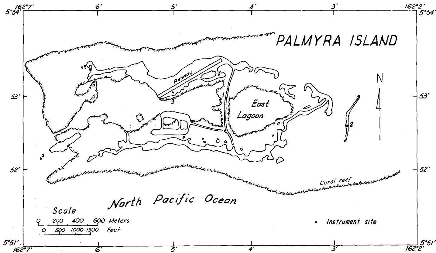
FIGURE 1.—Observation sites at Palmyra Island; 1) causeway site, 2) Barren Island site, 3) Army site.
