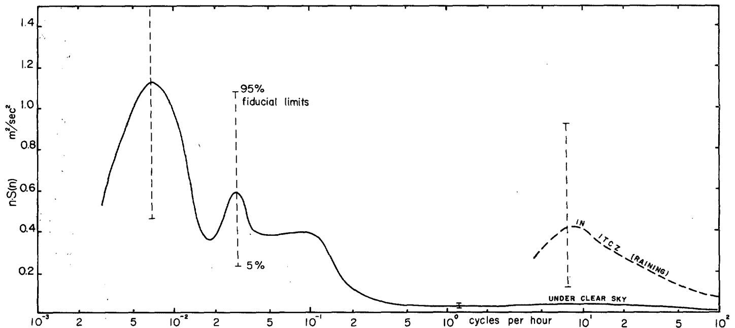
FIGURE 3.—Power spectra of surface wind speed at the causeway, Palmyra Island. The dashed line was based on data from a short period of precipitation during an ITCZ passage.
