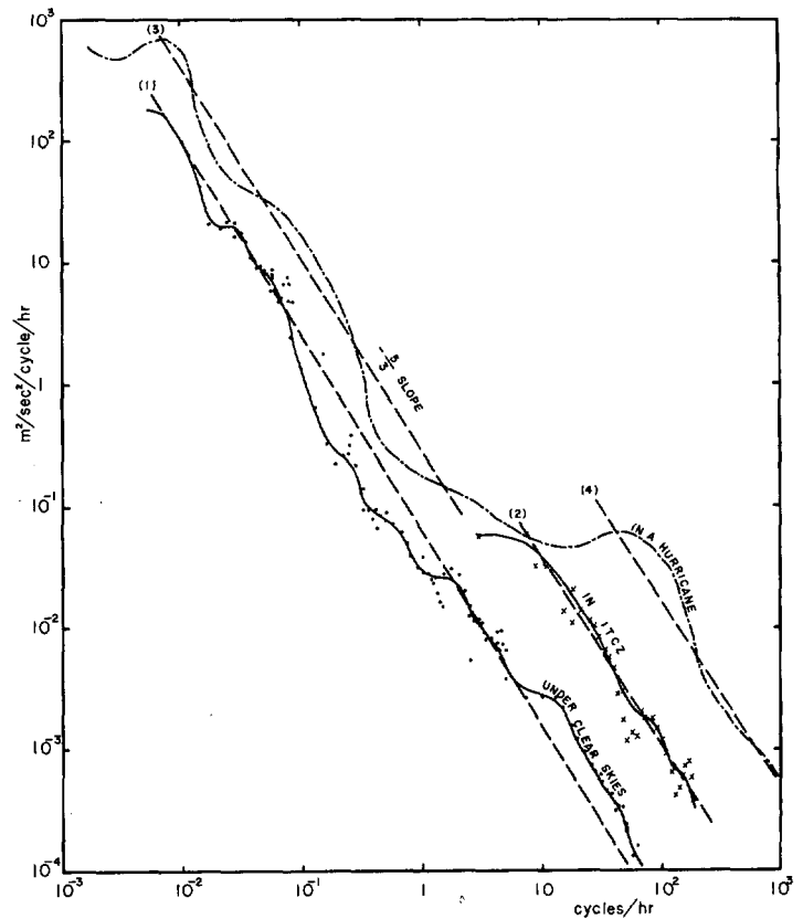
FIGURE 5.—Power spectrum of surface wind speed at the causeway, Palmyra Island (solid line), and Brookhaven, N.Y. (dot-dashed line). The ordinate is variance per frequency ( \text{m}^2/\text{sec}^2 ) ( \text{cycles/hr} ) -1 , the abscissa is frequency ( \text{cycles/hr} ), and both are plotted on a logarithmic scale. Long dashed lines are slope lines.
