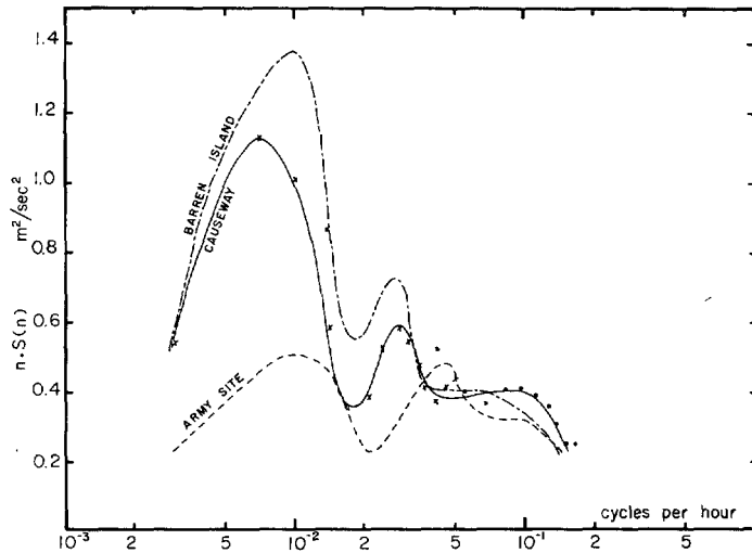
FIGURE 2.—Power spectra of surface wind speed recorded by MRI anemometer. The solid line is for causeway data, the dot-dashed line for Barren Island data, and the dashed line for Army site data.
