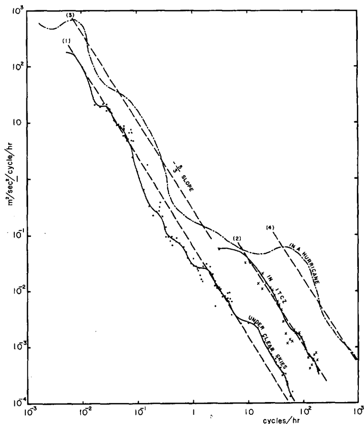
FIGURE 5.—Power spectrum of surface wind speed at the causeway, Palmyra Island (solid line), and Brookhaven, N.Y. (dot-dashed line). The ordinate is variance per frequency ( m^2/sec^2 ) (cycles/hr) -1 , the abscissa is frequency (cycles/hr), and both are plotted on a logarithmic scale. Long dashed lines are slope lines.
