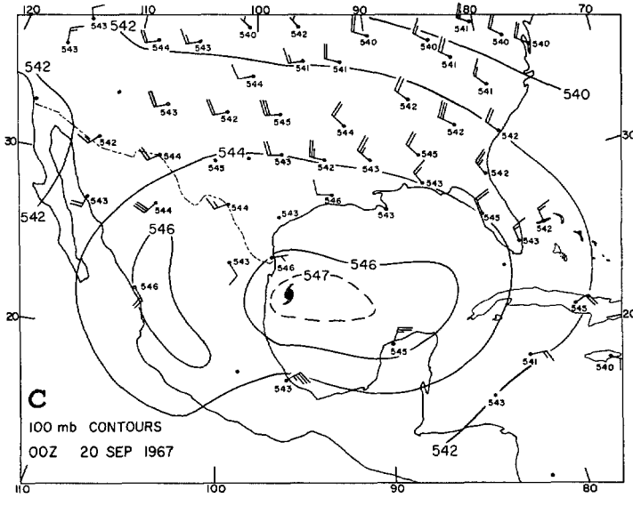
FIGURE 1.—(A) 300-mb contours and winds, (B) 300-mb isotherms, (C) 100-mb contours and winds, (D) 100-mb isotherms, and (E) 100-mb temperature departure from normal, all for 0000 GMT on Sept. 20, 1967. Contours in hundreds of feet; winds in knots; and isotherms and temperatures in degrees Celsius.
