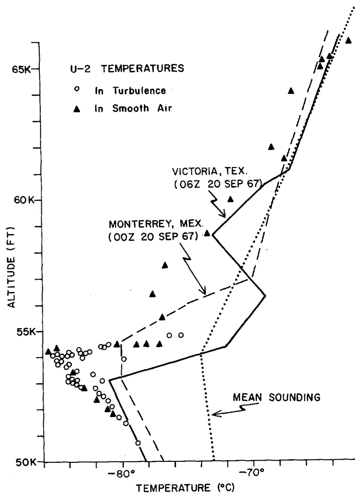
FIGURE 3.—Vertical distribution of temperature from aircraft measurements between 1605 and 1639 GMT on Sept. 20, 1967; temperature soundings for Monterrey, Mexico (0000 GMT on September 20), and Victoria, Tex. (0600 GMT on September 20), and the mean September sounding for the Caribbean are plotted for comparison.
