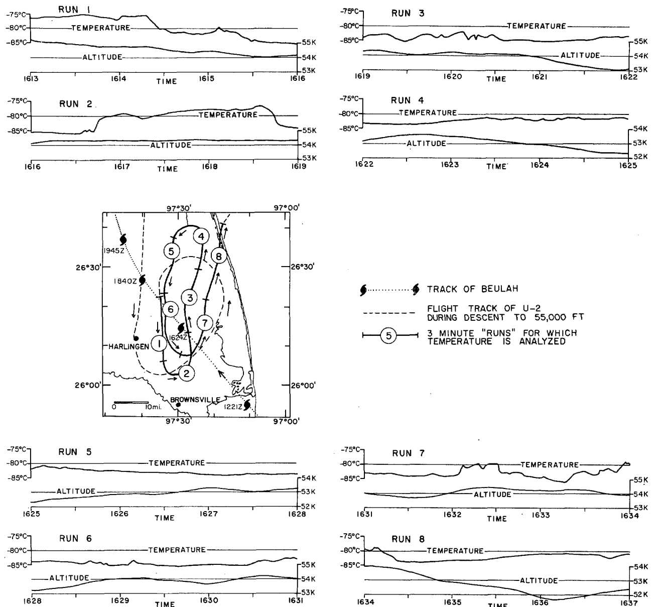
FIGURE 2.—Time histories of temperature (deg Celsius) and pressure altitude (feet) for runs 1 through 8 and the flight track of the U-2 aircraft over hurricane Beulah.
