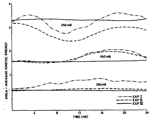
FIGURE 5.—Kinetic energy ( J \cdot cm^{-2} ) at selected levels for experiment I (dash-dot line), experiment II (dashed line), and experiment III (solid line).
