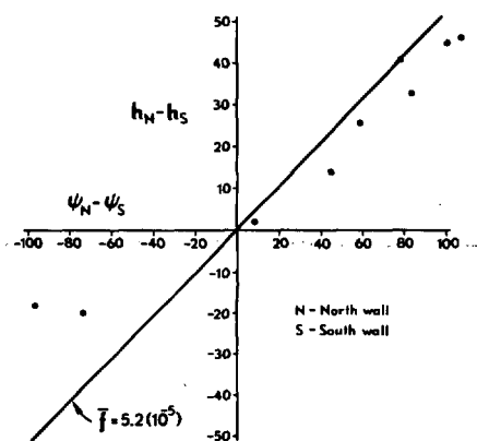
FIGURE 6.—Difference in stream function ( 10^{-5} \text{ m}^2 \cdot \text{s}^{-1} ) and heights ( h ) in meters between the north (N) and south (S) walls for experiment II. The solid line represents a geostrophic relation using the mean Coriolis acceleration for the channel.
