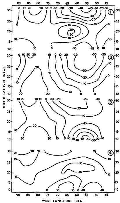
FIGURE 2.—Deviations from the initial 1000-mb height field (m) at: 1 hr (panel 1), 2 hr (panel 2), 3 hr (panel 3), and 4 hr (panel 4) from initial time of 1200 GMT on Aug. 29, 1965.
