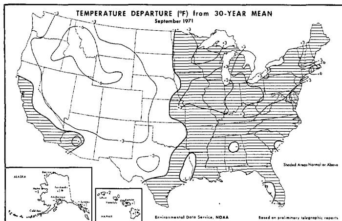
FIGURE 5.—Departure from normal of average surface temperature ( ^{\circ} F) for September 1971 (from Environmental Data Service and Statistical Reporting Service 1971).
