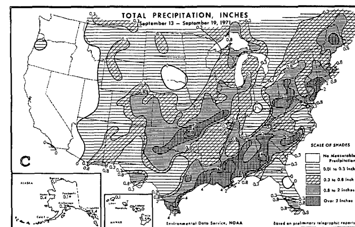
FIGURE 10—Same as figure 7, (A) for Sept. 14-18, 1971; (B) and (C) for Sept. 13-19, 1971.
