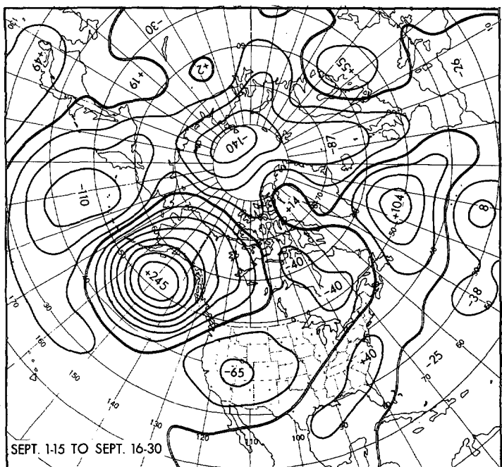
FIGURE 9.—Change in half-monthly mean 700-mb height (m) from Sept. 1-15 to Sept. 16-30, 1971.
