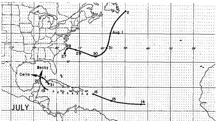
FIGURE 2.—Tracks of tropical depressions in 1970.
