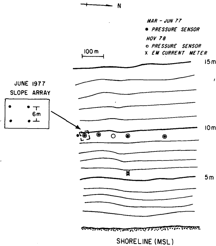
FIG. 2. Local bathymetry of Torrey Pines Beach and sensor locations for the two experiments. The contours were sampled in November 1978 and reported in Gable (1981).
