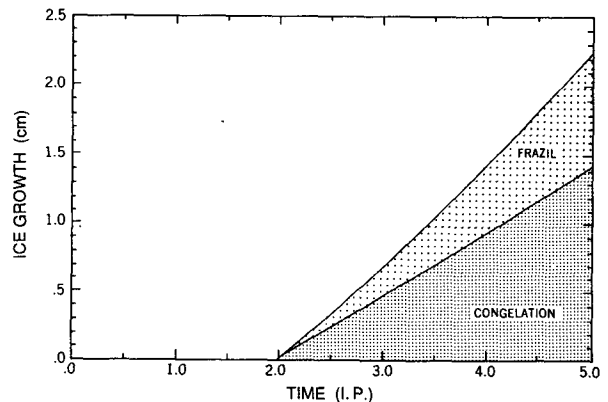
FIG. 6. Total ice production, using the YK sublayer. Congelation, or surface-cooled ice constitutes 1.4 cm of the total by 1.5 days after freezing begins. Frazil ice, formed due to the supercooling of water below the ice, constitutes 0.8 cm of the total by 1.5 days. Freezing is forced by a fixed surface heat sink of 60 \text{ W m}^{-2} . When the supercooling effect is not converted into equivalent frazil ice production, congelation ice production is nearly identical to that in this figure. When the Sheppard sublayer is used, the congelation ice total at five inertial periods is 2.4 cm, while the frazil ice total is only \sim 0.03 cm.
