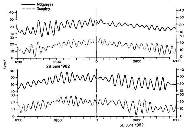
FIG. 9. Tide records from Magueyes Island and Guanica Harbor during the first field experiment in June 1982. Maximum seiche height exceeds the tidal range at both stations.
