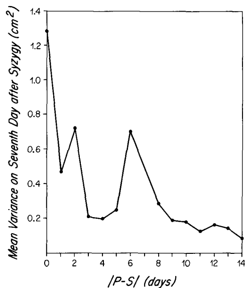
FIG. 5. Mean variance at seiche frequency on seventh day after syzygy in relation to absolute difference in time (days) between that syzygy and the nearest perigee ( |P - S| ). Seven days after perigean new or full moon ( |P - S| = 0 ), the mean variance is about ten times the value of the variance seven days after an apogean new or full moon ( |P - S| = 14 ).
