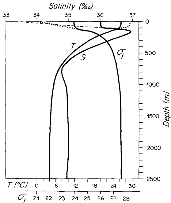
FIG. 7. Temperature, salinity and density ( \sigma_t ) profiles for a station offshore of Magueyes Island at 17°40'N, 67°00'W. Solid lines give values for late winter through early spring; dotted lines give values for late summer through early fall. Data from Fancher (1972).
