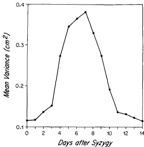
FIG. 4. Fortnightly distribution of sea-level variance at seiche frequency for Maguëyes Island based on a 10-year time series. Variance maximum occurs about one week after syzygy, i.e. new and full moon.
