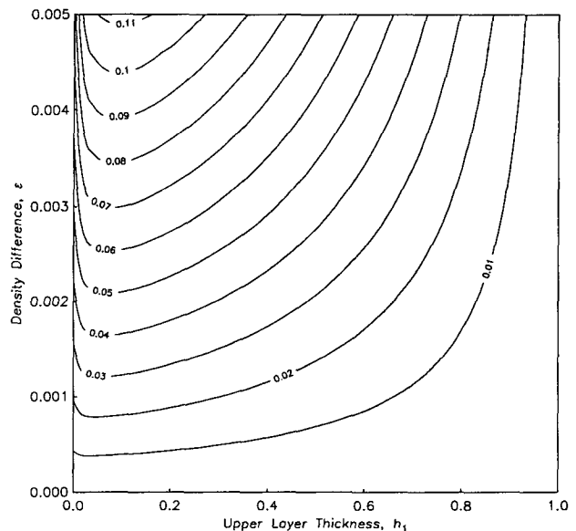
FIG. 4. Contours of the maximum shelf response |A|_{\max} for various density differences \epsilon and upper-layer thicknesses h_1 . Other parameters are d = 0.0045 , l = 0 .
