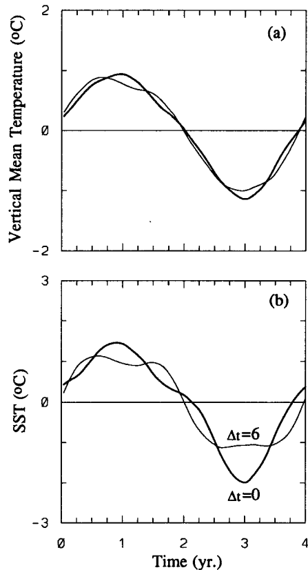
FIG. 7. Deviations from the mean annual cycle of the vertical-mean and sea surface temperatures as functions of time at 110°W on the equator. The thick lines are for the \Delta t = 0 experiment and the thin lines for the \Delta t = 6 experiment.
