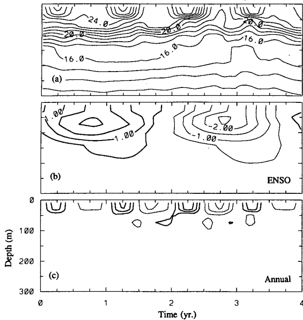
FIG. 6. Time–depth sections of (a) ocean temperature, its variations associated with (b) the interannual and (c) annual cycles (positive in bold and negative in thin lines) at 110°W on the equator: (b) is obtained by applying a 23-point running mean to the deviation (twice monthly) from the long-term mean profile to remove the annual variation; (c) is the residual of the total deviation from (b). Contour intervals are 1°C in (a) and (c) and 0.5°C in (b).
