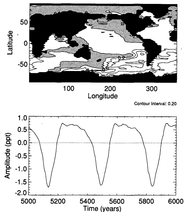
FIG. 6. EOF mode 1 for the surface salinity field, \mathcal{F}(0.8) case. Top: normalized eigenvector. Bottom: eigenamplitude (ppt) as a function of time. EOF 1 corresponds to the freshwater cap that forms in the Ross Sea during times of reduced convection.
