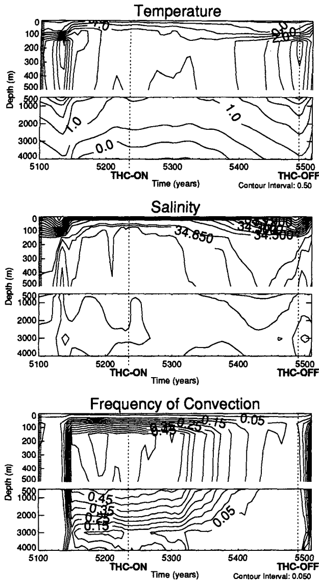
FIG. 9. Time versus depth contours of model fields averaged over the Weddell Sea, \mathcal{F}(0.8) case. Top: temperature ( ^{\circ}\text{C} ), showing the subsurface (200–500 m) heating that destabilizes the water column. Middle: salinity (psu), showing the freshwater cap that forms, shutting off convection. Bottom: Frequency of convection (fraction of grid-boxes).
