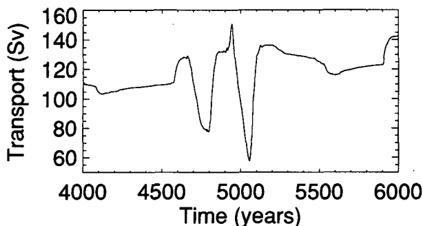
FIG. 22. Drake Passage transport (Sv) for case \mathcal{F}(1.1) , where the P - E field has been multiplied by 1.1.
