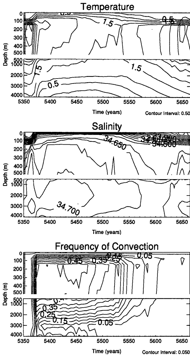
FIG. 20. Time versus depth contours of model fields averaged over the Weddell sector, \mathcal{F}(0.8) case. Top: temperature ( ^{\circ}\text{C} ), showing the subsurface (200–500 m) heating that destabilizes the water column. Middle: salinity (psu), showing the fresh water cap that forms, shutting off convection. Bottom: frequency of convection (fraction of gridboxes).
