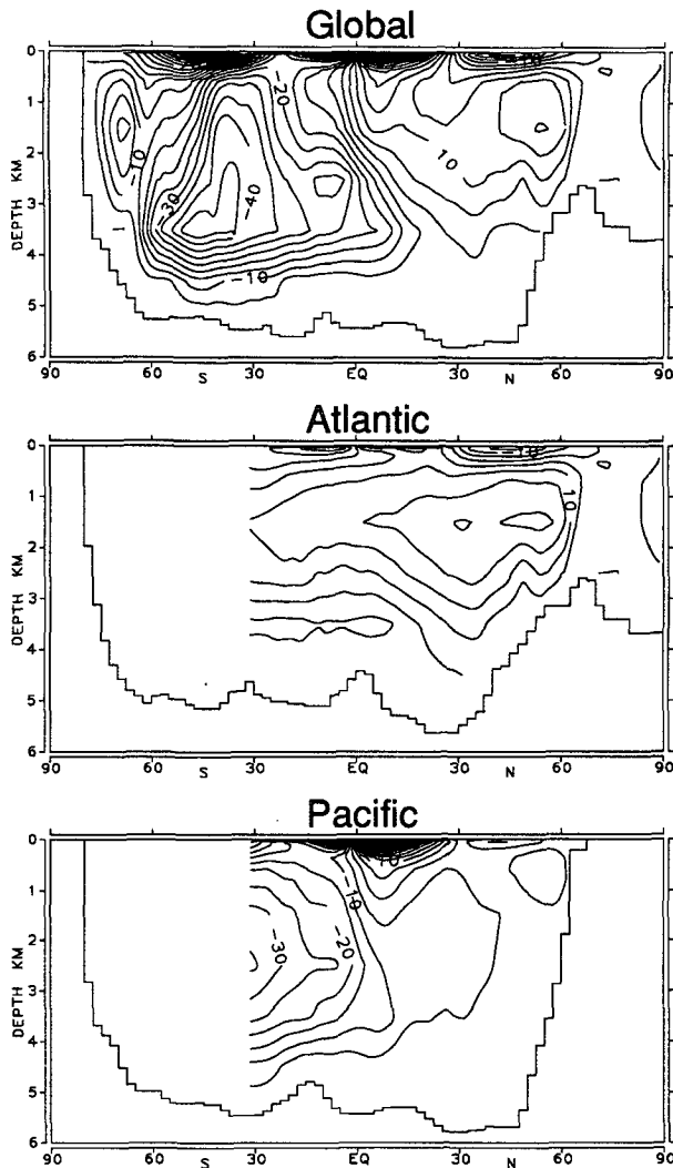
FIG. 3. Meridional circulation (Sv) for case \mathcal{F}(0.8) at time THC-ON, the peak of Southern Ocean thermohaline activity. Top panel: all oceans. Middle panel: Atlantic. Bottom panel: Pacific. Contour interval is 5 Sv.
