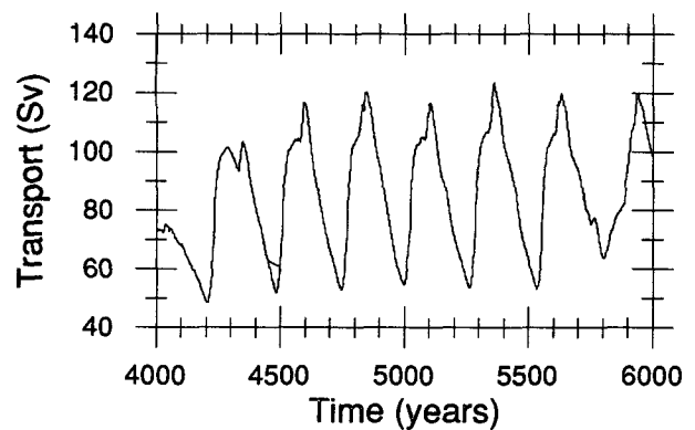
FIG. 26. Drake Passage transport (Sv) for the test case using a quadratic equation of state. Unlike the cases with a linearized equation of state, oscillations develop readily.
