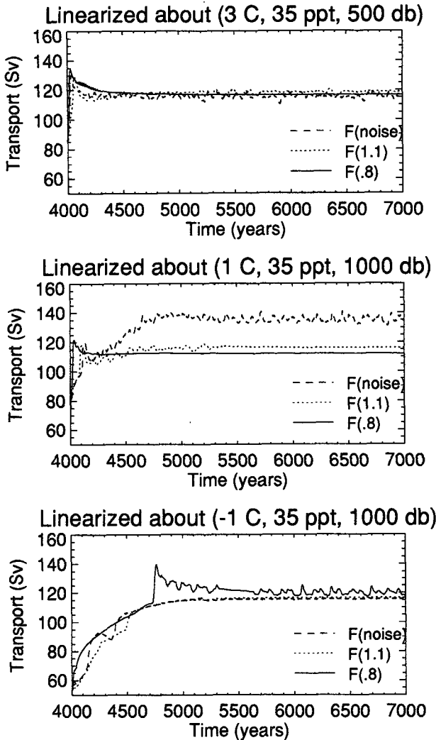
FIG. 25. Drake Passage transport for nine cases with a linearized equation of state: in none of the cases were the large-scale fluctuations seen.
