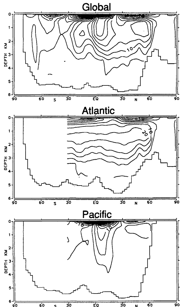
FIG. 4. Meridional circulation (Sv) for case \mathcal{F}(0.8) at model year THC-OFF, the minimum of Southern Ocean thermohaline activity. Top panel: all oceans. Middle panel: Atlantic. Bottom panel: Pacific. Contour interval is 5 Sv.
