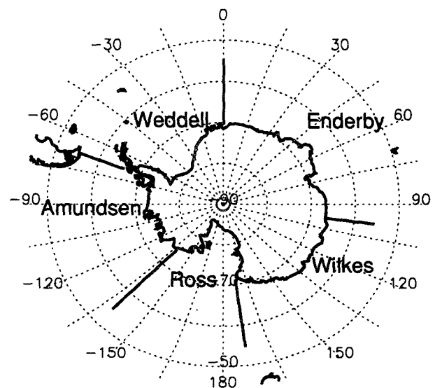
FIG. 12. Antarctic zones used for the analysis. All zones extend to 60°S.
