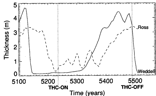
FIG. 15. Average sea ice thickness (m) in the Weddell and Ross sectors as a function of time, \mathcal{F}(0.8) case.
