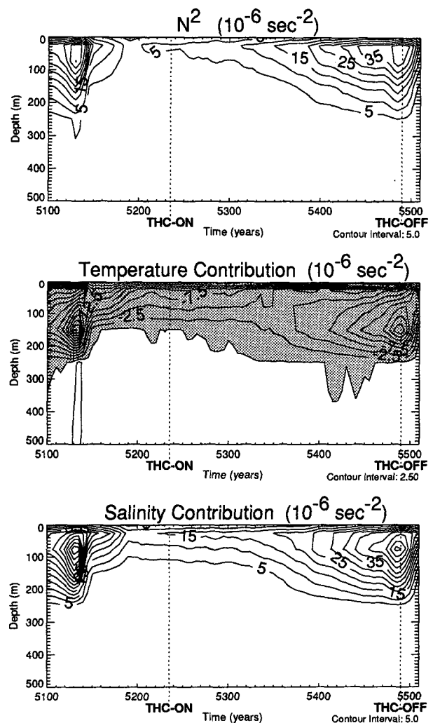
FIG. 10. Evolution of the stability of the Weddell Sea water column, \mathcal{F}(0.8) case. Top: total N^2 . Middle: the (destabilizing) contribution due to temperature. Bottom: the (stabilizing) contribution due to salinity. Negative regions are shaded; only the top 500 m are shown. Units are 10^{-6} \text{ s}^{-2} .
