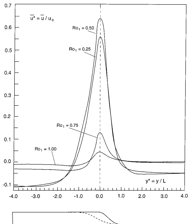
FIG. 16. Normalized along-isobath mean velocity profiles for the streamwise location x^* = 1 for Ro = 0.08 and a range of Ro_1 ; that is, for the same experiments as illustrated in Figs. 15a–d.
