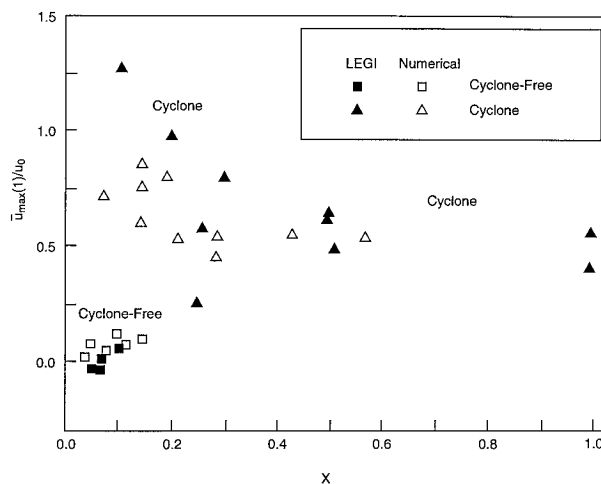
FIG. 17. Plot of the normalized maximum mean velocity obtained at x^* = 1 against the normalized tidal excursion; open symbols indicate numerical runs and closed symbols LEGI physical model experiments.
