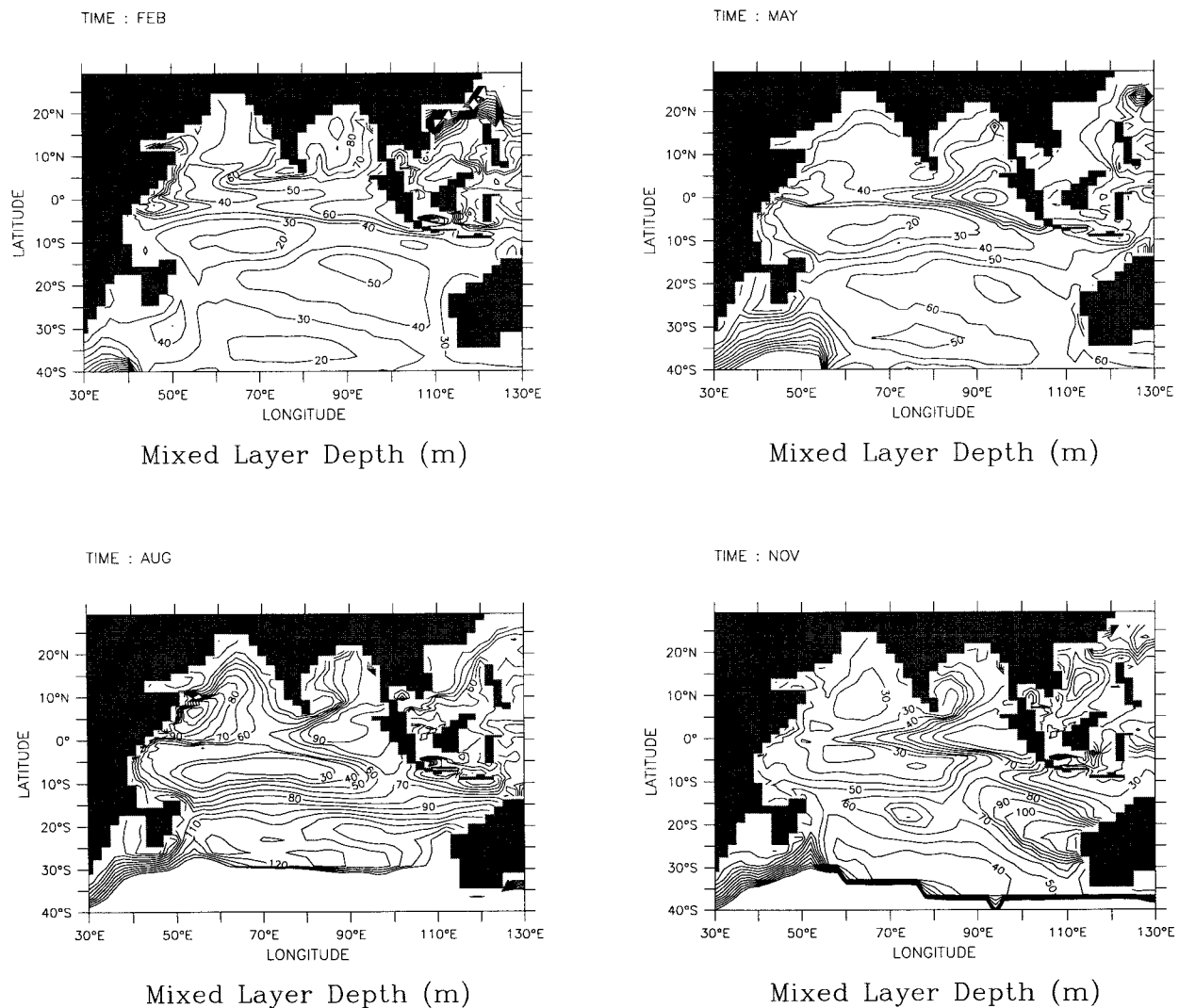
FIG. 8. Mixed layer depths of experiment SF for (a) February, (b) May, (c) August, and (d) November. The MLD was defined by the depth at which temperature is 1^{\circ}\text{C} less than that of the top level (7.5 m). C.I. = 10 m.
