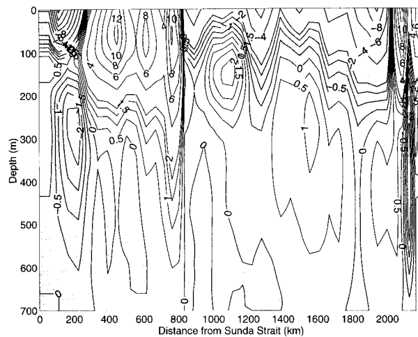
FIG. 13. Annual mean geostrophic velocity (0/700 m) across IX1 section from XBT data using T - S relation from Levitus and Boyer (1994) projected onto XBT line. Shaded areas denote flow from the Indian to Pacific Oceans. Units are \text{cm s}^{-1} .
