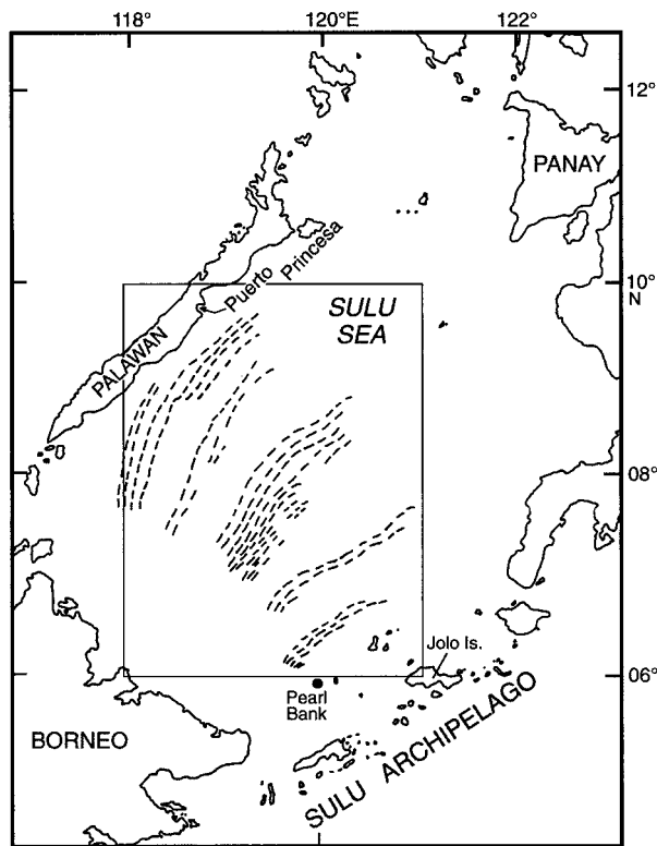
FIG. 1. Location of Palawan Island, the Sulu Sea, and the Sulu Archipeligo in the Philippines. Dashed lines represent the surface expression of internal solitons that are generated by strong tides near Pearl Bank and that travel northwestward, reaching Puerto Princesa in about 2.5 days (after Apel et al. 1985).
