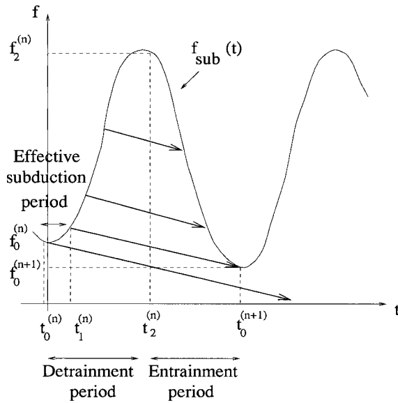
FIG. 2. Schematic of the outcrop line displacement (24), shown as a cosinelike curve, and associated time and f coordinate. In the course of year n , the latitude reached by columns subducting during the detrainment period [t_0^{(n)}, t_1^{(n)}] is indicated by the arrows. Only columns subducted before t_1^{(n)} reach the permanent thermocline. Note the variable position of the outcrop line from one winter to the next.
