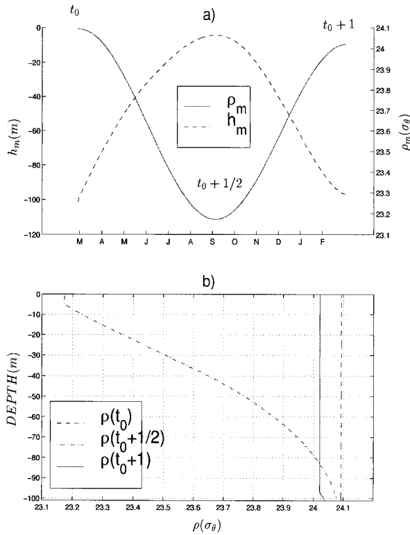
FIG. 5. (a) Evolution of the mixed layer depth (in m) and density (in \sigma_\theta ) along the 1-yr trajectory for the column initially located at 21.2°N. The x axis denotes time, in month. (b) Density profile at times t_0 , t_0 + 1/2 , and t_0 + 1 .
