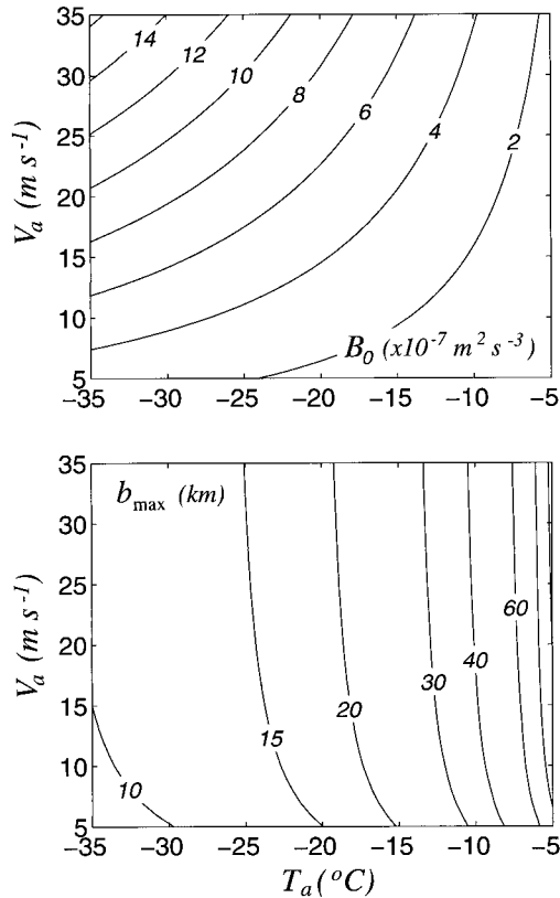
FIG. 2. Surface buoyancy flux B_0 (upper) and maximum polynya width b_{\max} (lower) from the Pease polynya model with constant forcing, computed using (11) and (13) with various air temperatures T_a and offshore wind speeds V_a .
